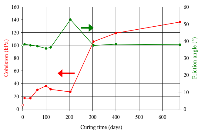
Figure 5: Evolution of the shear resistance parameters with time (treated silt from Soumagne, Belgium, PI=16). The white points at t=0 are related to the untreated specimen.
