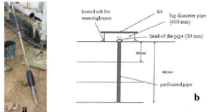
Figure 12: Double-packer probe used for variable head Nasberg test (a); schematic view of the constant head Nasberg method (b).
