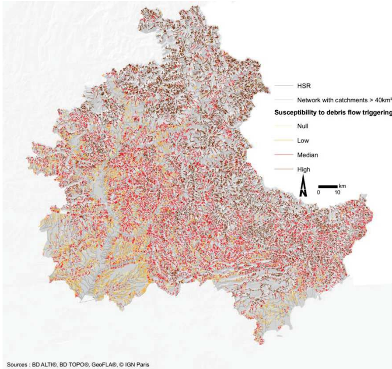
Fig 2: Map of susceptibility to debris-flow activity within the triggering areas.
