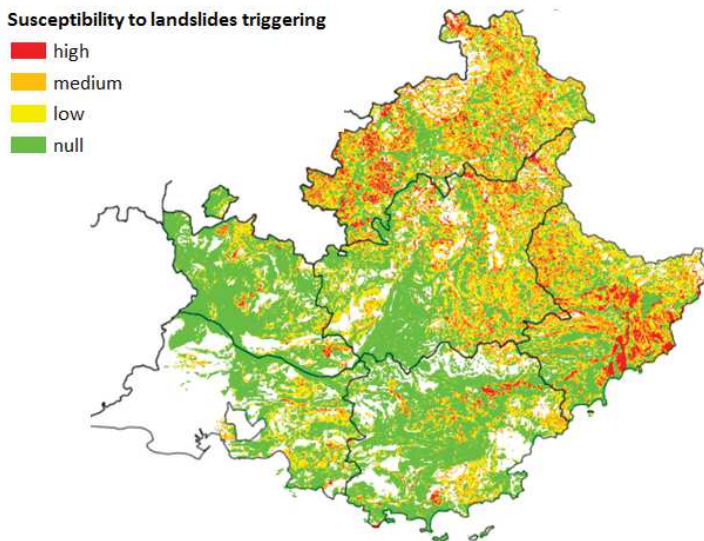
Fig 3: Map of the susceptibility to landslides triggering, taking into account the number of observed events since 1900 in each homogeneous geotechnical area and susceptibility factors.
