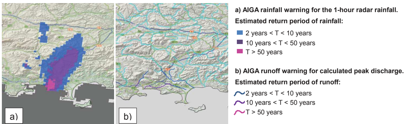
Fig 1: AIGA warnings emitted at 16:00 the 26/10/2012 during a storm event in the neighborhood of Toulon city, southern France. (a) : Estimated return periods for the 1-hour radar rainfall. (b) Estimated return periods for the peak flow discharge computed by the hydrological model. The pixel size is 1 km 2 .
