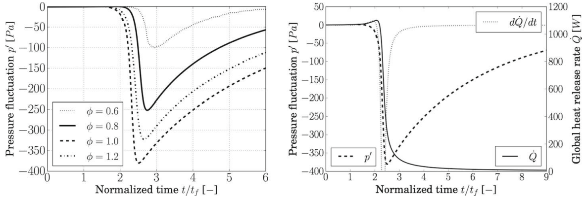
Fig. 4 Left : Pressure fluctuation profiles for the different equivalent ratios \phi recorded at probe P_{ff} . The wall temperature is T_w = 300 K for all equivalence ratios. Right : Evolution of pressure fluctuation, global heat release and the rate of change of the heat release for the stoichiometric flame using complex chemistry
