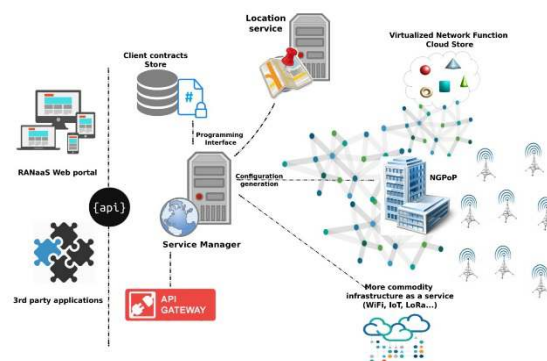
Fig. 6. RANaaS overall architecture
