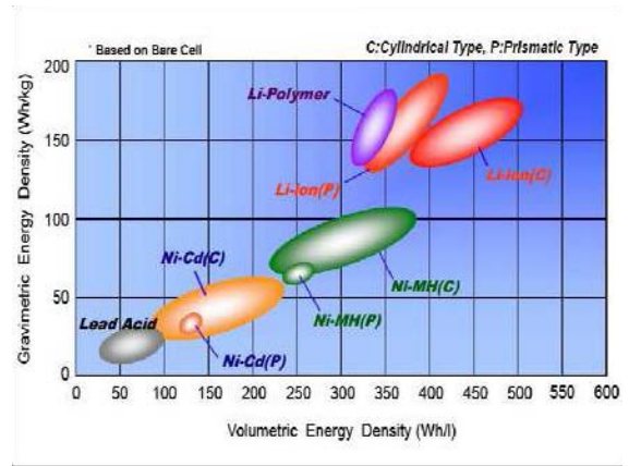
Fig. 6. General view of battery technology in term of energy density (based on DoE approach) – Note : NiZn is similar to NiMH in density)
