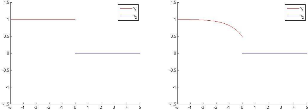
(a) The value function with entry cost c_2 \geq \frac{1}{\lambda} = 1 . (b) The value function with entry cost c_2 = \frac{1}{2} < 1 = \frac{1}{\lambda} .
