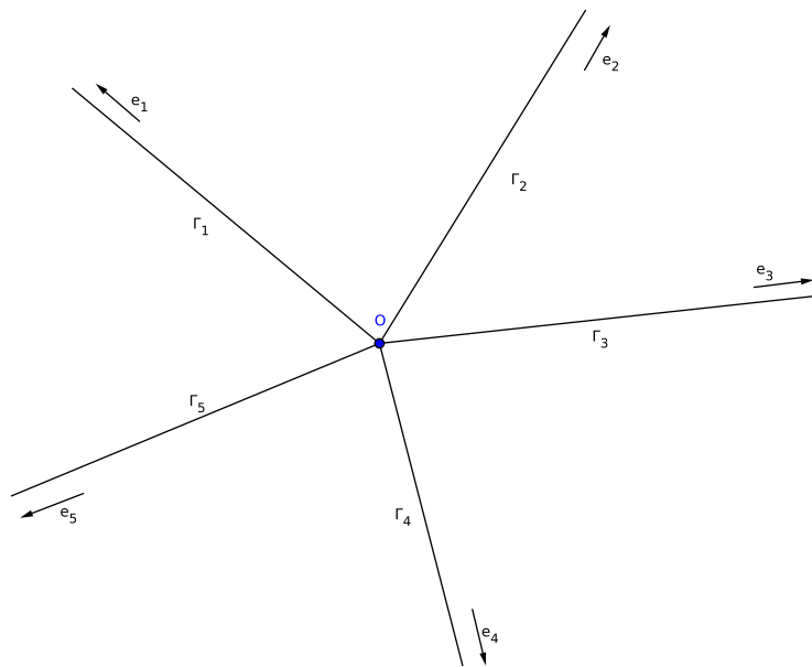
Figure 1: The network \mathcal{G} ( N = 5 )
