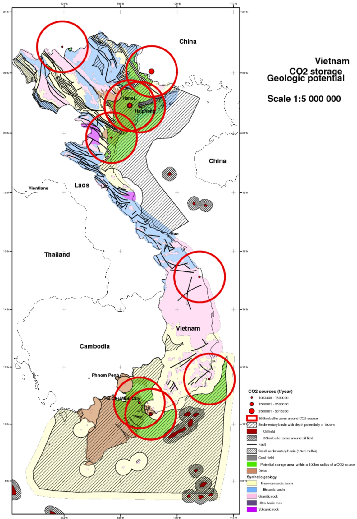
Figure 2: Geological formations potentially favorable for CO 2 storage in Vietnam (BRGM/TKV 2009, 34)
