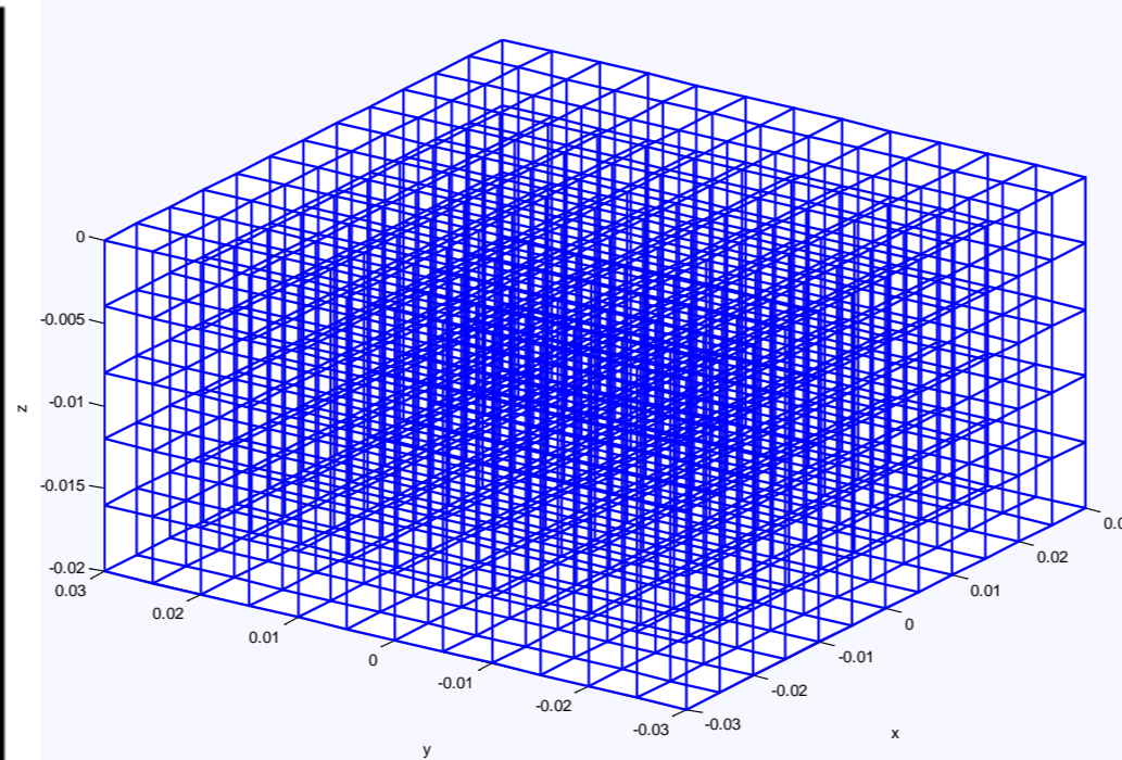
Hexaedral Mesh of the plate part
