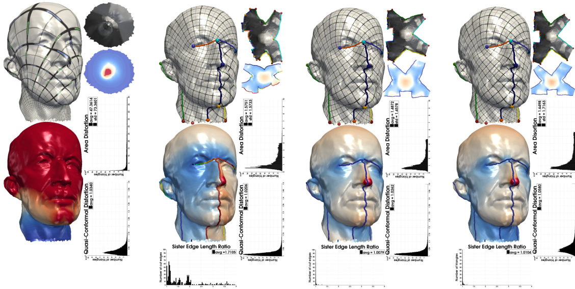
(a) LSCM [Lev02] (b) LSCM [Lev02], conic cuts (c) Our approach (d) Our approach - Seamless
