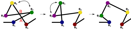
Figure 6: Possible cut intersections are recursively resolved by cone swapping. Here, the intersection A between segments [\theta_1, \theta_2] and [\theta_4, \theta_5] is first solved instead of intersection B because it counts the most intersections between its two extremities \theta_1 and \theta_5 .
