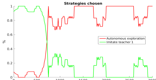
Fig. 7: Evolution of the choice of learning strategy of SGIM-ACTSCL: percentage of times each strategy is chosen across time
