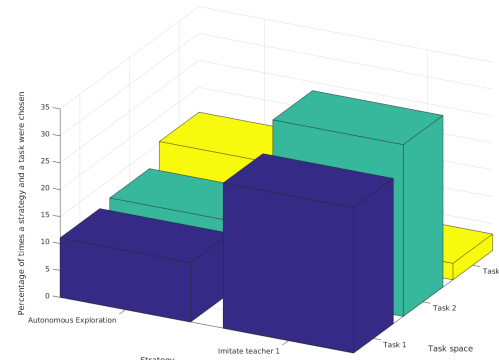
Fig. 9: Synergy between the choice of task space and the choice of learning strategy of SGIM-ACTSCL: percentage of times each strategy and task is chosen over all the learning process
