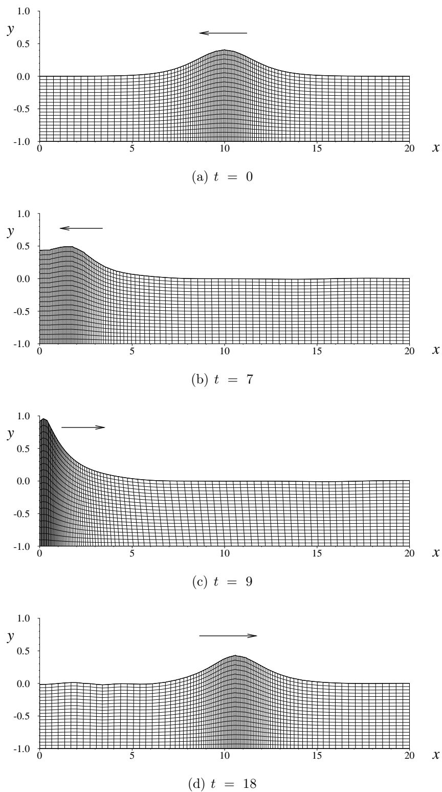
Figure 6. Solitary Wave (SW) interaction with a vertical fixed wall at different instances of time. SW's amplitude is \alpha = 0.4 . The propagation direction is shown with a horizontal arrow.
