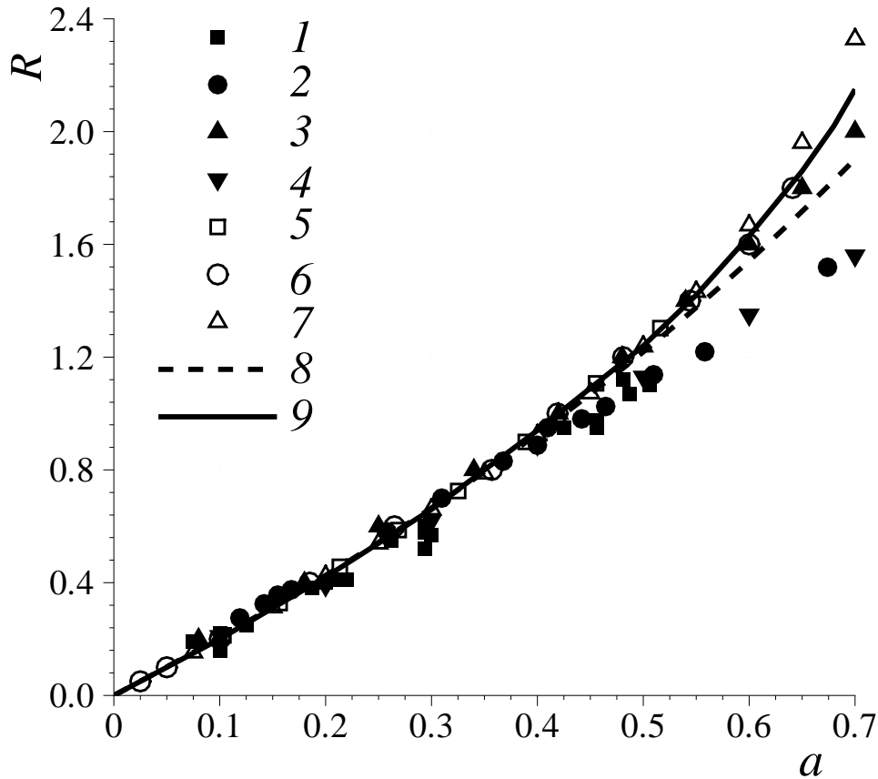
Figure 7. Dependence of the maximal run-up \mathcal{R}_{\max} at the vertical wall on the incident solitary wave amplitude \alpha . Experimental data: (1) [79], (2) [57], (3) [16], (4) [56]. Numerical data: (5) [34], (6) [8], (7) [10]. Analytical prediction [74] (8) (dashed line). The present study (9) is given by the solid line.
