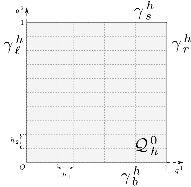
Figure 3. Sketch of the discretized reference domain \mathcal{Q}_h^0 .
