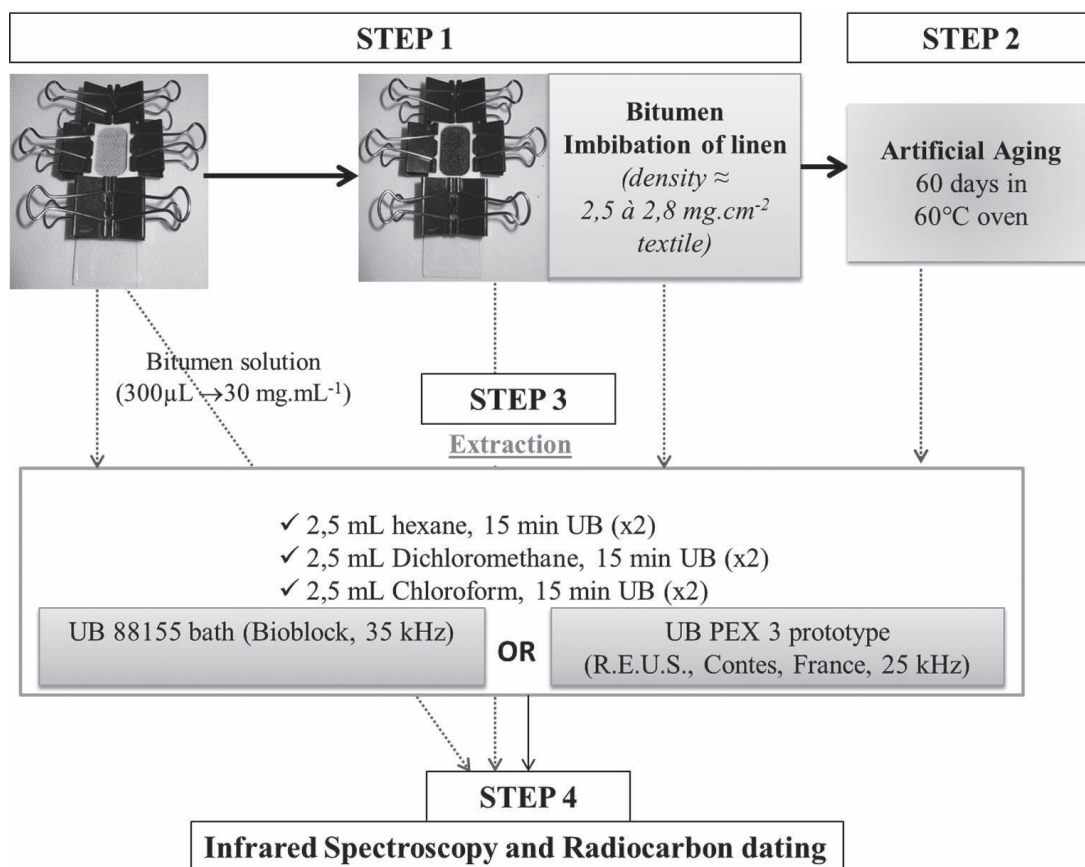
Figure 2: Experimental protocol developed to prepare, extract and analyze the modern linen textile/ bitumen test-sample. It divides into four steps.
