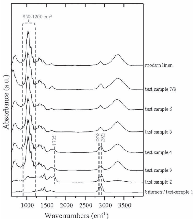
Figure 7: ATR-IR spectra obtained on test-samples 2, 3, 4, 5, 6 and 7/8 compared to pure linen and bitumen ones. Test-samples 2, 3 and 4 (steps 1, 2, 3) spectra have a shoulder at 1705\text{ cm}^{-1} and the double band characteristic of bitumen in the peak 2800\text{-}3000\text{ cm}^{-1} is not clearly identifiable, but could not be excluded. On the contrary, test-samples 5 and 6 (steps 1, 2) have IR spectra very similar to those of pure line spectra: no shoulder at 1705\text{ cm}^{-1} and a single broad band in the peak 2800\text{-}3000\text{ cm}^{-1} .
