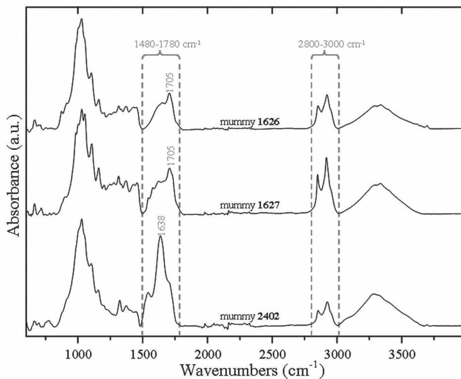
Figure 4: Representative ATR-IR spectra obtained on textile samples from embalmed mummies 1626, 1627 and Predynastic mummy 2402, underlining a different signature for samples where bitumen is suspected. General profiles are similar for textile taken on embalmed mummies 1626 and 1627. They are characterized by a large peak around 1480-1780 \text{cm}^{-1} with a single band close to 1705 \text{cm}^{-1} ; and a double band around 2800-3000 \text{cm}^{-1} . Mummy 2402 profile is slightly different: the single band in the first peak has a lower wavenumber at 1638 \text{cm}^{-1} and the double band in the 2 800-3 000 \text{cm}^{-1} region is less intense.
