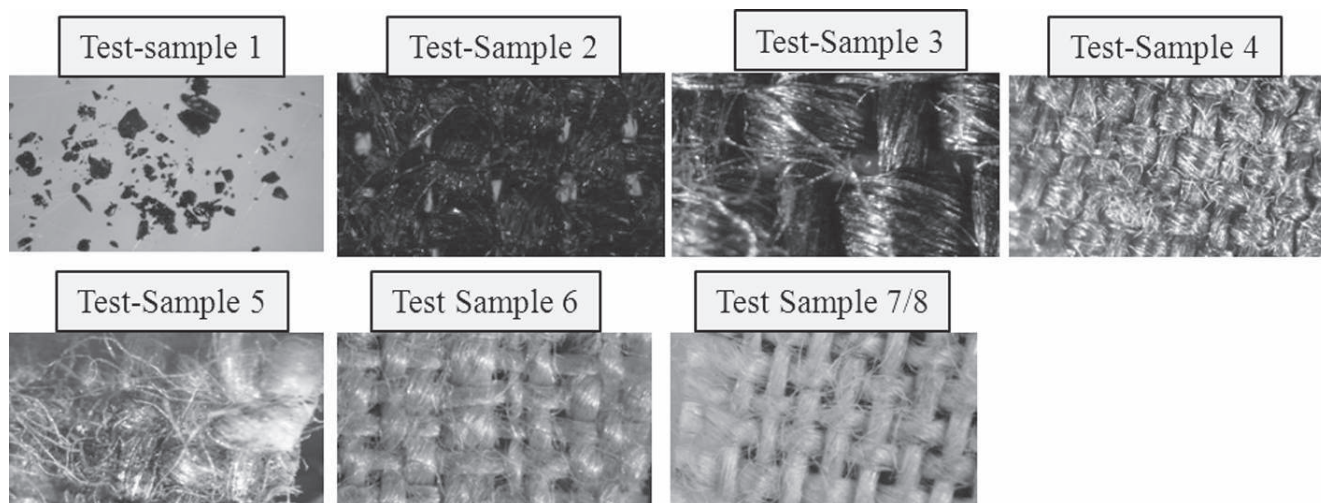
Figure 6: (See colour plate) Binocular microscopy observations of the eight test-samples. Test-sample 7 and 8 have not been dipped in bitumen (7: modern linen; 8: modern linen which undergone the extraction protocol [step 3]). Test-sample 2 shows the linen textile after being dipped in bitumen (step 1). Test-samples 3 and 4 have been dipped in bitumen, thermally degraded and extracted (steps 1, 2, 3); they seem more blackened and brighter than test-samples 5 and 6, which have been dipped in bitumen and extracted without being thermally degraded (steps 1, 2).
