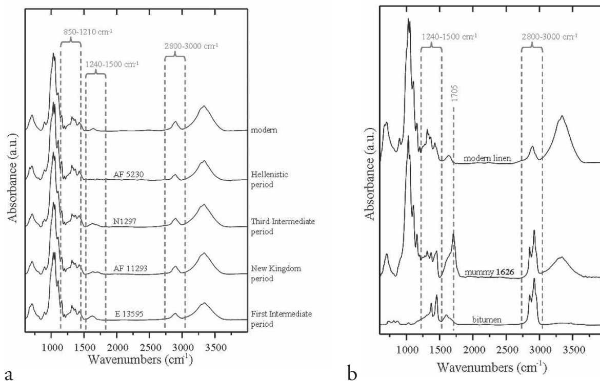
Figure 5: (a) IR spectra obtained for the pure linen textiles held at the Département des Antiquités égyptiennes of the Louvre Museum, and radiocarbon dated from the First Intermediate Period (E 13595) to the Hellenistic Period (AF 5230). The five IR spectra are quasi-similar (b): Comparison of the IR spectra obtained on one pure modern linen textile, on a textile from an embalmed mummy (1626) and on Judean bitumen. The double band in the 2800-3000 \text{cm}^{-1} peak is visible on the embalmed mummy textile as well as on the bitumen spectrum, but is indiscernible on the "pure" linen textile spectrum. Besides, the single band close to 1705 \text{cm}^{-1} is absent of both the bitumen and the pure linen spectra.
