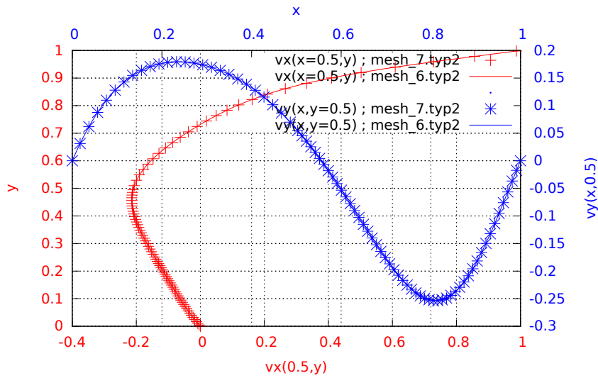
Fig. 4 Velocity profiles for \nu = 1/100
