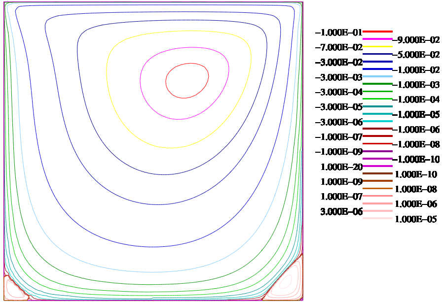
Fig. 3 Streamlines for \nu = 1/100 (mesh_5)
