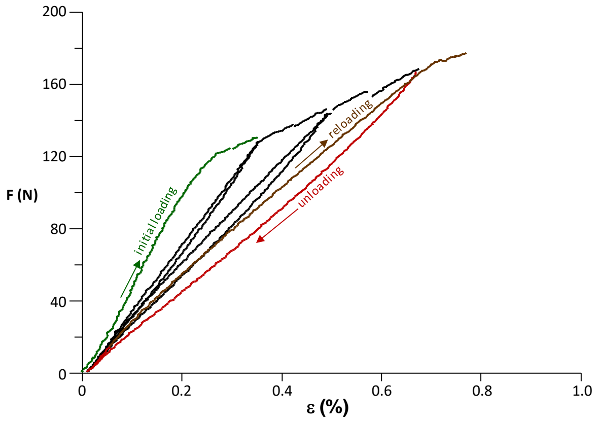
Figure 3: Tensile force-strain curve with unload-reload cycles for the minicomposites (for clarity only a few hysteresis loops are represented).
