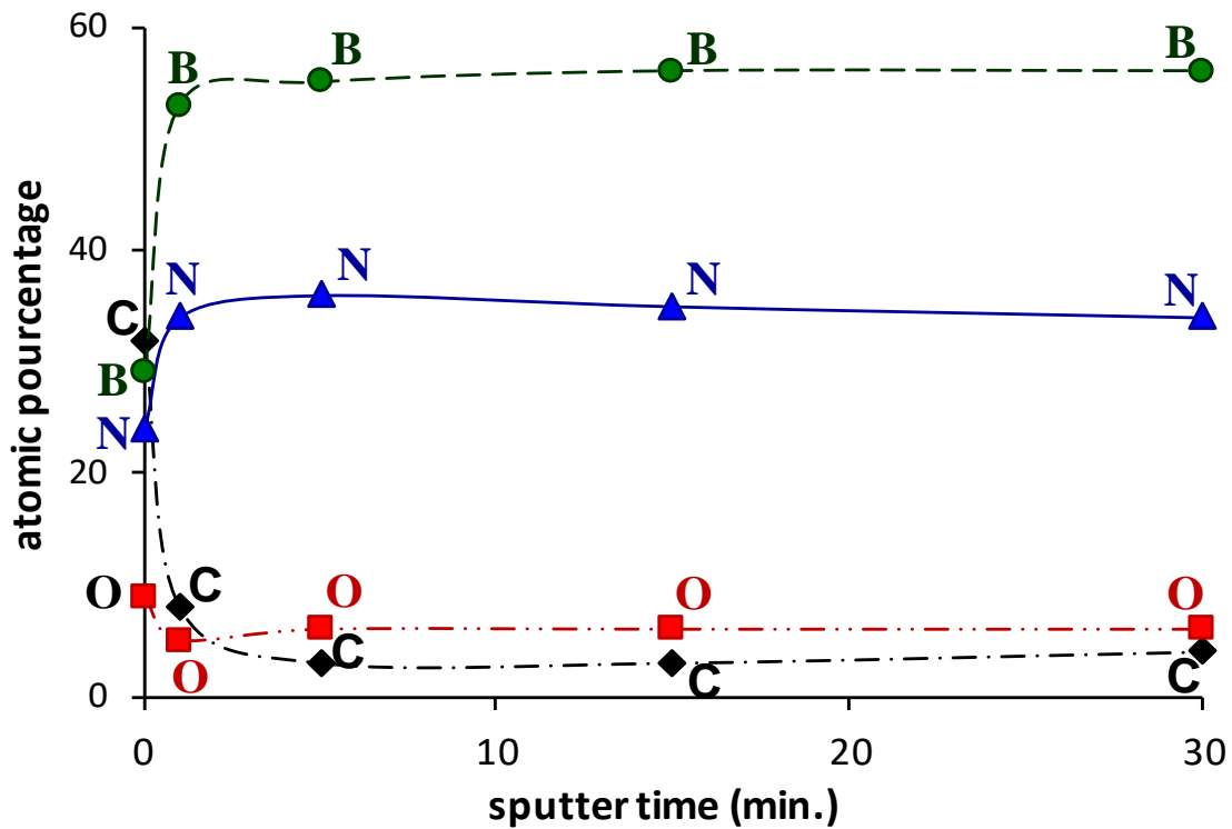
Figure 2: XPS depth atomic concentration profiles for the BN film (sputter rate: ~ 1 - 4 nm/min).
