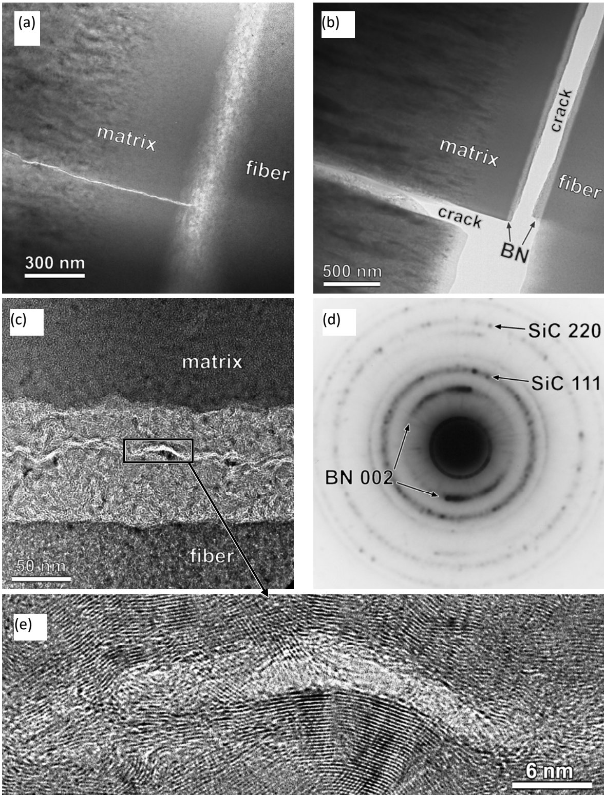
Figure 4: TEM observation of the SiC/BN/SiC minicomposite according to the BF mode (a), (b) and (c), the SAED technique (negative pattern of the Hi-Nicalon fiber and the interphase) (d) and the HR mode (e).
