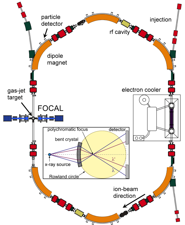
FIG. 1. Schematic view of the ESR storage ring and the location of the FOCAL spectrometer at the gas-jet target. In the upper left dipole magnet a particle detector recording down-charged ions is used to apply a coincidence condition on the x-ray spectra. The inset shows a schematic view of the FOCAL crystal-optics layout.
