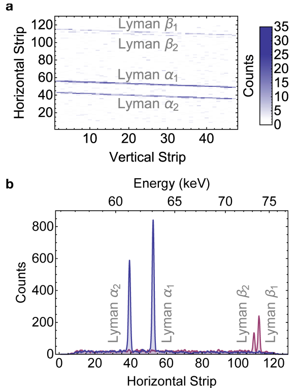
FIG. 2. (a) Coincident x-ray spectrum as recorded by one of the FOCAL spectrometers. (b) Spectrum of the Lyman- \alpha and - \beta doublets of \text{Au}^{78+} obtained by a projection of the respective two-dimensional intensity distribution shown in (a).
