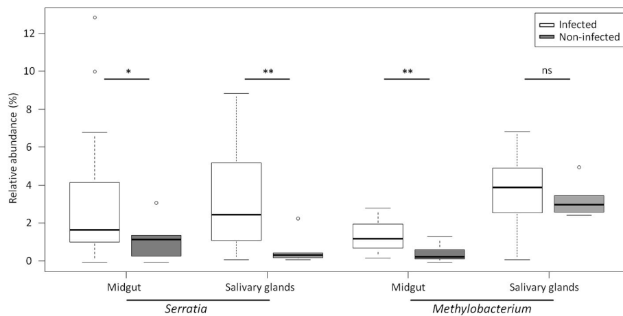
FIGURE 5 | Relative abundance of Serratia and Methylobacterium in P. falciparum infected and P. falciparum non- infected mosquitoes for both salivary glands and midgut. The boxes represent the interquartile range (25–75th percentile), and the line within each box corresponds to the median value. * P < 0.05 , ** P < 0.01 , and ns, non-significant. Circles represent outliers.
