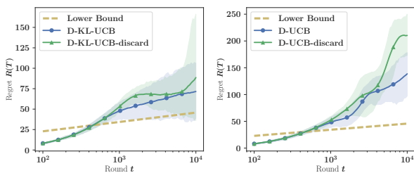
Figure 2: Expected regret of D-UCB and D-KLUCB in the censored setting vs the equivalent discarding policies when \mu = 500 and m = 1000 . Results are averaged over 200 independent runs.
