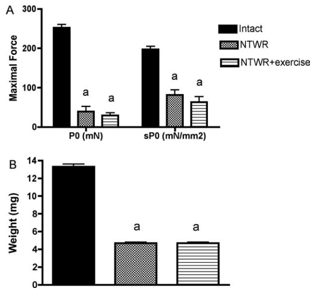
FIGURE 1. Absolute ( P_0 ) and specific ( sP_0 ) maximal forces (A) and weight (B) of soleus muscles 1 month after nerve transection without possible repair. Values are mean \pm SEM. Number per group = 10–12. NTWR, nerve transection without possible repair. a Significantly different from intact ( P < 0.05 ).
