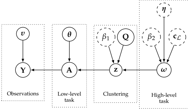
Figure 1: Directed acyclic graph of the proposed hierarchical Bayesian model. (User-defined parameters appear in dotted circles).
