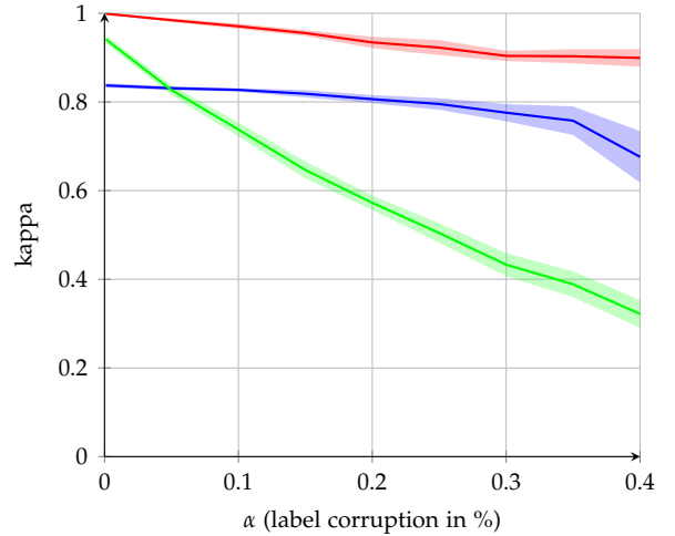
Figure 4: Classification accuracy measured with Cohen's kappa as a function of label corruption \alpha : proposed model (red), MDA with abundance vectors (blue) and MDA with measured reflectance (green). Shaded areas denote the intervals corresponding to the standard deviation computed over 20 trials.
