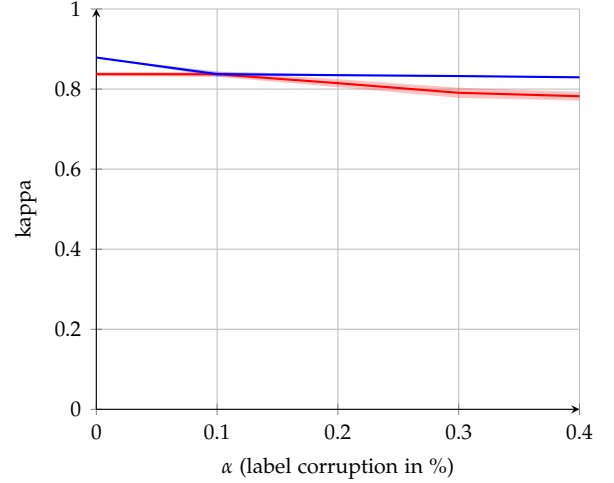
Figure 7: Real MUESLI image. Classification accuracy measured with Cohen's kappa as a function of label corruption \alpha : proposed model (red), random forest (blue). Shaded areas denote the intervals corresponding to the standard deviation computed over 10 trials.
