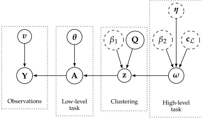
Figure 1: Directed acyclic graph of the proposed hierarchical Bayesian model. (User-defined parameters appear in dotted circles).
