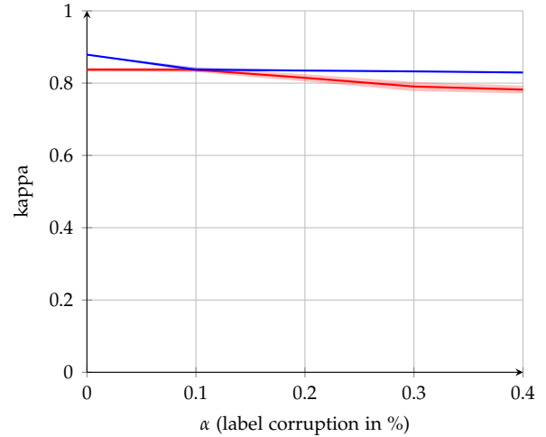
Figure 7: Real MUESLI image. Classification accuracy measured with Cohen's kappa as a function of label corruption \alpha : proposed model (red), random forest (blue). Shaded areas denote the intervals corresponding to the standard deviation computed over 10 trials.
