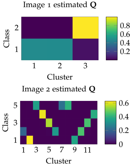
Figure 5: Estimated interaction matrix Q for Image 1 (top) and Image 2 (bottom).
