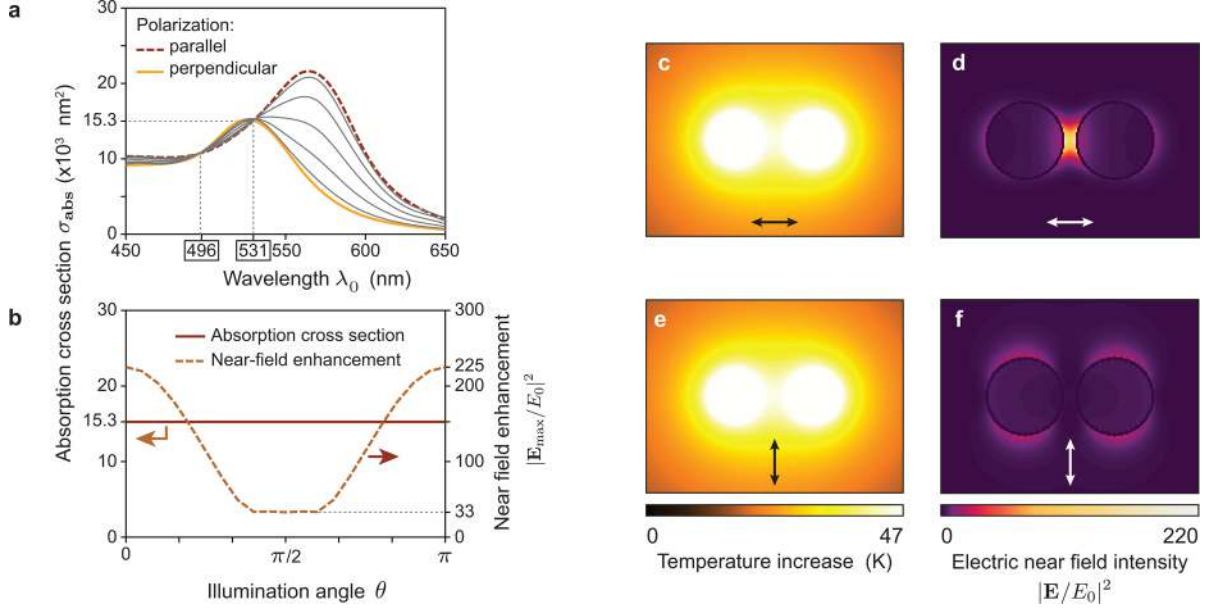
Figure 1. (a) Absorption cross section of a dimer structure composed of two 60 nm gold spheres in water separated by a 10 nm gap, for longitudinal and perpendicular polarizations of the incident light. Gray lines correspond to intermediate polarization angles ( 15^\circ , 30^\circ , 45^\circ , 60^\circ , and 75^\circ ). A crossing is observed for the isosbestic wavelengths \lambda = 496 and 531 nm. (b) Absorption cross section and normalized electric near-field as functions of the illumination angle, at the isosbestic wavelength \lambda = 531 nm, identified in (a). (c) Temperature map for a longitudinal polarization of the incident light and an arbitrary light irradiance of 1 \text{ mW}/\mu\text{m}^2 . (d) Corresponding normalized electric near-field. (e, f) Same as (c) and (d) for a perpendicular incident light polarization.
