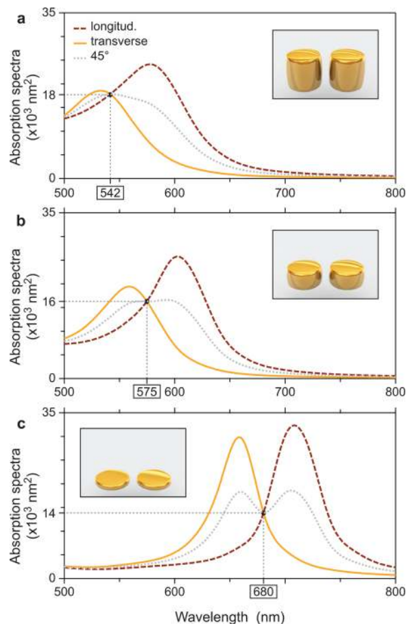
Figure 6. Calculations of cross-polarization absorption spectra using the BEM for different gold disc-dimer thicknesses e : (a) e = 60 nm, (b) e = 30 nm, and (c) e = 10 nm. Insets represent the morphology of the structures. The illumination axis is vertical on these insets. Dashed lines correspond to calculations with light polarization parallel to the axis of the dimer. Solid lines correspond to light polarization perpendicular to the dimer axis. Dotted lines correspond to an intermediate light polarization ( 45^\circ ).
