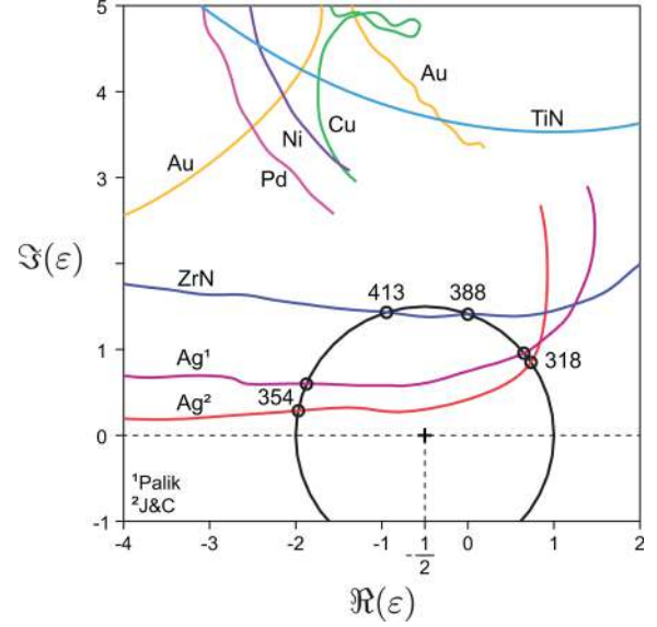
Figure 3. Polar plots of the complex permittivity of common plasmonic materials. The condition given by eq 11 is represented as a solid line circle. Only materials crossing this circle can exhibit isosbestic conditions in the quasistatic regime.
