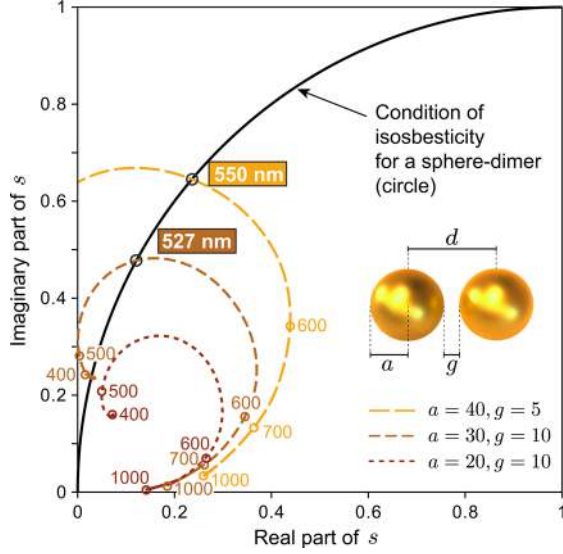
Figure 2. Space of \underline{s} values for a gold sphere-dimer in water in the complex space. The black solid line represents the values that \underline{s} must equal to obtain an isosbestic sphere-dimer. Dashed lines represent the actual values of s as a function of the wavelength from \lambda = 400 to \lambda = 1000 nm, for three different gold sphere-dimer morphologies ( a, g ). Particular wavelength values have been indicated, in particular the isosbestic wavelength (boxed numbers).
