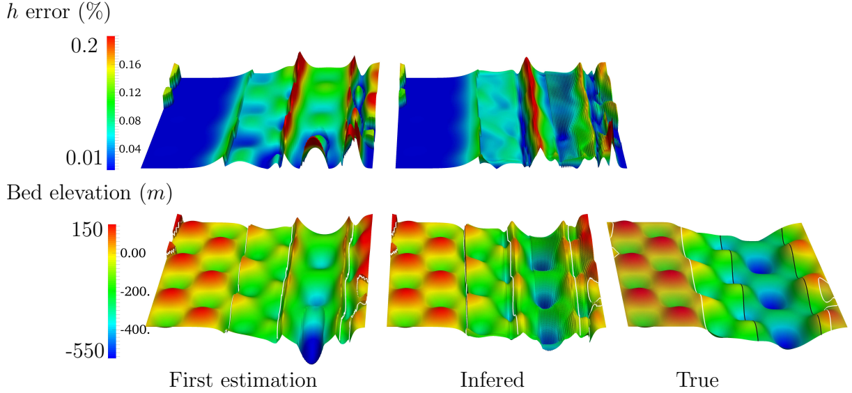
Figure 9: Test case 1 with exact measurements: bed elevation. (Down) From left to right: “1st guess”= value from (19), inferred value after VDA#2, true value. (Top) Corresponding relative errors. The white lines denotes the sub-regime area boundaries defined from Table 1.
