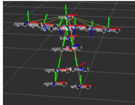
Fig. 3. Skeleton frames.
