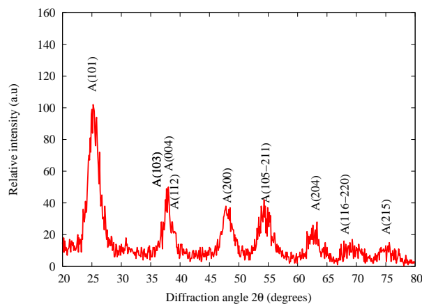
Figure 1. X-ray diffraction of the TiO 2 grafted acetylacetone nanopowder.
