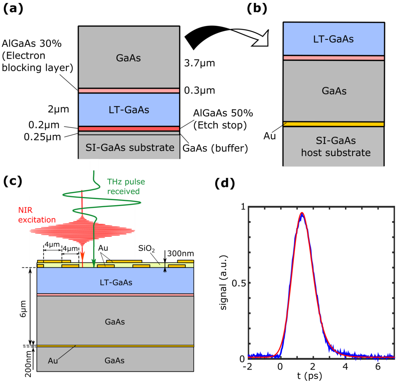
Fig. 1 (a) LT-GaAs growth. The MBE growth sequence on a SI GaAs substrate consists of: i) a 250-nm-thick GaAs buffer; ii) a 200-nm-thick AlGaAs (50%) etch stop layer; iii) 2- \mu\text{m} -thick LT-GaAs ; iv) 300 nm of AlGaAs (30%); and, v) 3.7 \mu\text{m} of GaAs. (b) Pre-photolithography sample. The MBE grown sample is wafer bonded to a gold-coated host SI GaAs substrate. The substrate and the AlGaAs (50%) layer of the MBE grown wafer are removed, exposing the LT-GaAs active region with the echo-blocking metal plane 6 \mu\text{m} below the surface. (c) Schematic diagram of iPC switch, with interdigitated gold electrodes on top of the LT-GaAs layer consisting of 4- \mu\text{m} -wide electrodes, each separated by 4 \mu\text{m} . The THz pulse and the femtosecond pulse are focused on the front face of the switch, generating carriers in the LT-GaAs layer with the THz induced current collected from the switch contacts. (d) Experimental measurement of carrier lifetime in the LT-GaAs active layer (blue line). The red line is a numerical fit, showing a lifetime of \sim 400 fs.
