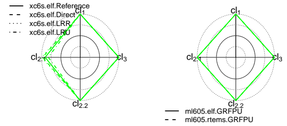
(a) Different cache replacement policies (bench. matmult on the GR-XC6S without RTEMS). (b) Impact of the RTOS: without and with RTEMS (benchmark lms on the ML605).
