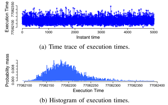
Fig. 6. Time trace and histogram of execution times (benchmark cnt on the GR-XC6S reference architecture without RTEMS).
