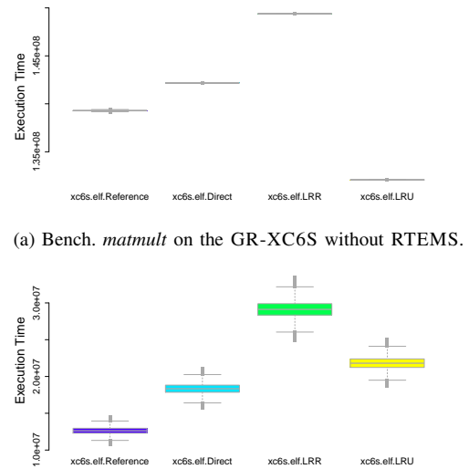
Fig. 7. Box plots of execution times for different cache replacement policies.
