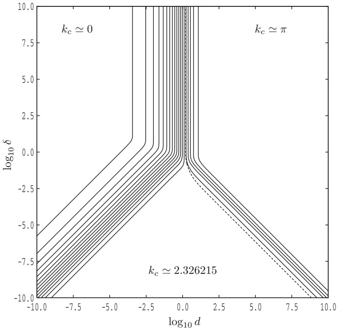
Fig. 7 Contours of Ra_c and k_c as functions of \log_{10} d and \log_{10} \delta . Integer values of Ra_c are used, while 20 equal intervals between 0 and \pi are used for k_c . The dotted lines correspond to the CT/CHF case, Ra_c = 27.097628 and k_c = 2.326215
