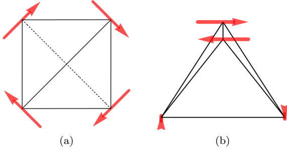
FIG. 12: Spin configuration in the 4-sublattice Palmer–Chalker phase, \Psi_4 , transforming with the T_2 irrep of T_d : (a) viewed along [001] axis; (b) viewed slightly off the [110] axis. At the phase boundary with the \Psi_2 phase, each of the six Palmer–Chalker ground states can be transformed continuously into a \Psi_2 state.
