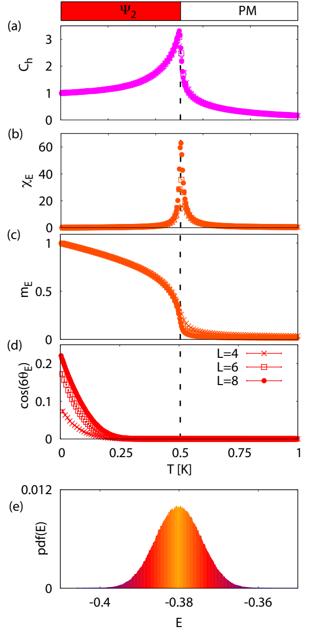
FIG. 18: Finite-temperature phase transition from the paramagnet into the non-coplanar antiferromagnet \Psi_2 , as determined by classical Monte Carlo simulation of \mathcal{H}_{\text{ex}} [Eq. (1)], for parameters appropriate to \text{Er}_2\text{Ti}_2\text{O}_7 26 , i.e. J_1 = 0.11 \text{ meV} , J_2 = -0.06 \text{ meV} , J_3 = -0.1 \text{ meV} setting J_4 = 0 \text{ meV} . a) Temperature dependence of the specific heat c_h(T) . b) Temperature dependence of the order-parameter susceptibility, \chi_E(T) . c) Temperature dependence of the order parameter, |\mathbf{m}_E(T)| . d) Temperature dependence of the secondary order parameter, \cos 6\theta_E . e) Probability distribution of the energy E evaluated at the transition temperature for a system of size L = 12 . The black dashed line indicates a continuous phase transition at T_N = 505 \pm 5 \text{ mK} . Simulations were performed for clusters of N = 16L^3 spins, with L = 4, 6, 8, 12 .
