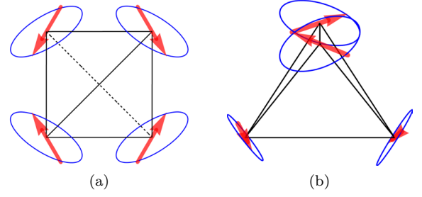
FIG. 9: Example of a spin configuration within the one-dimensional manifold of states transforming with the E irrep of T_d : (a) viewed along [001] axis; (b) viewed slightly off the [110] axis. The manifold possesses 4-sublattice long-range order, with spins lying in the “XY” plane perpendicular to the local [111] axis at each site. The manifold is continuous, and can be parameterised with a single angle \theta_E . The manifold can be generated by a clockwise rotation of all spins around their respective local axes.
