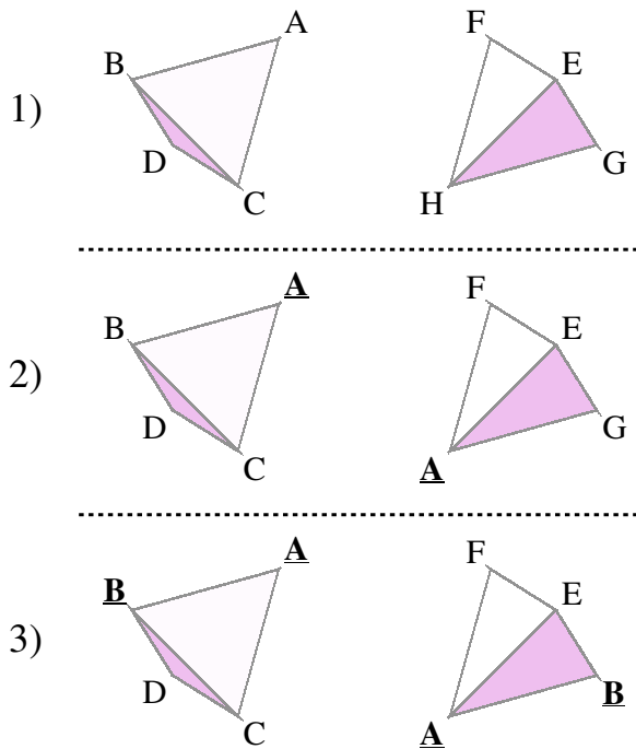
FIG. 6: The “Lego-brick” rules describing how the ground states of a single tetrahedron can be connected to tile the pyrochlore lattice. The two tetrahedra in the left and right panels represent a pair of tetrahedra in distinct ground-state configurations. Distinct spin orientations on the sites of each tetrahedron are denoted by letters a – h . Three cases are shown. In case (1) all of the ground states for a single tetrahedron have different spin orientations for any given site. This means that two tetrahedra in distinct ground states cannot be joined together because they do not share a common spin orientation on any site. In this case the 4-sublattice ground state of the lattice is unique with q = 0 order, up to global symmetry operations. In case (2) there are two ground states configurations for a tetrahedron which share a common spin orientation on a single site, here denoted a . These tetrahedra can be joined together by sharing the spin in orientation a . In this case the ground state of the lattice has a degeneracy of at least \mathcal{O}(2^L) . Indeed, successive kagome layers of spins can be independently in BDC or FEG configurations. In case (3) there is a pair of ground states which share common spin orientations on two sites, here denoted a and b . These tetrahedra can be joined together by sharing the spin in orientation a or the spin in orientation b . In this case the ground state of the lattice has a degeneracy of at least \mathcal{O}(2^{2L}) .
