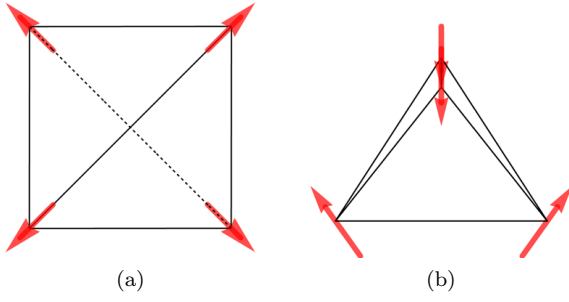
FIG. 10: Spin configuration in the 4-sublattice non-coplanar antiferromagnet, \Psi_2 , selected by fluctuations from the one-dimensional manifold of states transforming with \mathbf{E} : (a) viewed along [001] axis; (b) viewed slightly off the [110] axis. At the phase boundary with the Palmer–Chalker phase, each of the six \Psi_2 ground states can be transformed continuously into a Palmer–Chalker state without leaving the ground-state manifold.
