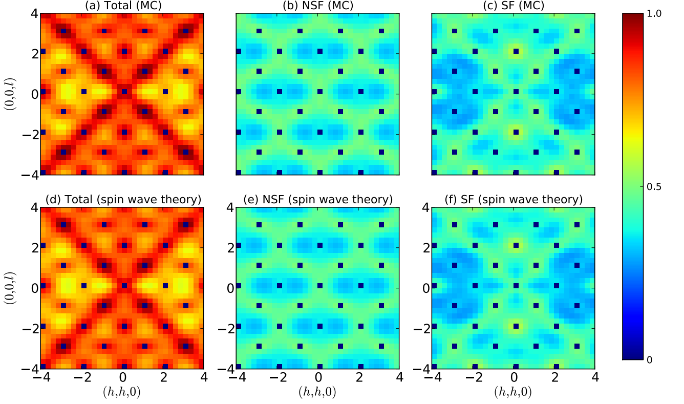
FIG. 20: Comparison between results for equal-time structure factor S(\mathbf{q}) obtained in classical Monte Carlo (MC) simulation and classical low-temperature expansion (spin wave theory) for parameters appropriate to \text{Yb}_2\text{Ti}_2\text{O}_7 43 . a) Total scattering in the (h, h, l) plane within MC simulation. b) Associated scattering in the non spin-flip (NSF) channel. c) Associated scattering in the spin-flip (SF) channel. d) Total scattering in the (h, h, l) plane within a spin-wave expansion about the ferromagnetic ground state. e) Associated scattering in the NSF channel. f) Associated scattering in the SF channel. Rods of scattering in the (h, h, h) direction, associated with a low-energy spin-wave excitation [cf. Fig. 25], are visible in both SF and NSF channels. All results were obtained at T = 0.05 K, for exchange parameters J_1 = -0.09\text{meV} , J_2 = -0.22\text{meV} , J_3 = -0.29\text{meV} , setting J_4 = 0 . SF and NSF channels are defined with respect to a neutron with polarisation in the (1, -1, 0) direction, as in Ref. 89. S(\mathbf{q}) has been calculated using the experimentally measured g-tensor for \text{Yb}_2\text{Ti}_2\text{O}_7 43,90 , with g_z = 1.77 , g_{xy} = 4.18 . In order to avoid saturating the colour scale, the intensity associated with Bragg peaks at reciprocal lattice vectors has been subtracted.
