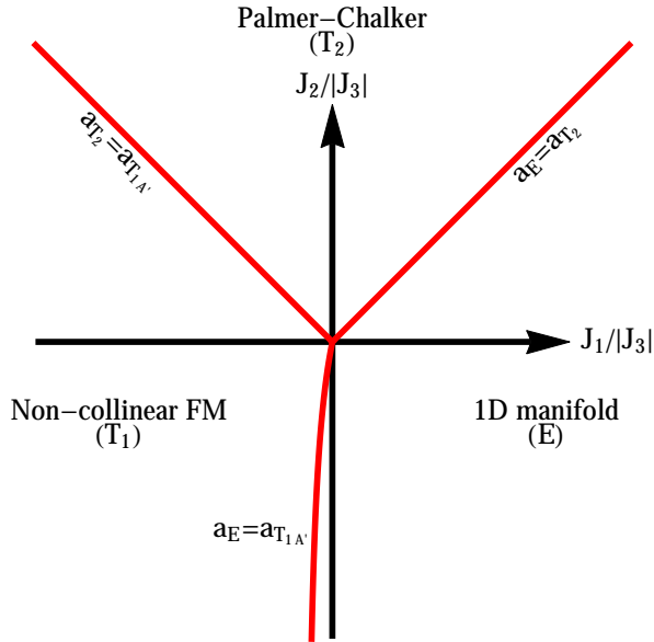
FIG. 7: Classical ground state phase diagram of \mathcal{H}_{\text{ex}} [Eq. (4)] for J_3 < 0 , J_4 = 0 , as a function of (J_1, J_2)/|J_3| . In the absence of fluctuations, the ground states are a non-collinear FM transforming with the T_1 irrep of T_d ; a one-dimensional manifold of states transforming with the E irrep of T_d ; and the Palmer–Chalker phase, a coplanar antiferromagnet transforming with the T_2 irrep of T_d . All three phases have long-range 4-sublattice order. Analytical expressions for the boundaries between phases are given in Eq. (28–30), with coefficients a_\lambda defined in Table V.
