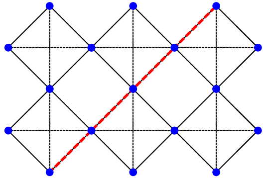
FIG. 13. A path (in red) between two spins on the checkerboard lattice containing only nearest neighbour \mathcal{J}_1 bonds. The correlation function between two such spins in the disordered regime is calculated in section D 3.
