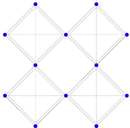
FIG. 12. The checkerboard lattice formed by the set of B-spins on the shuriken lattice.
