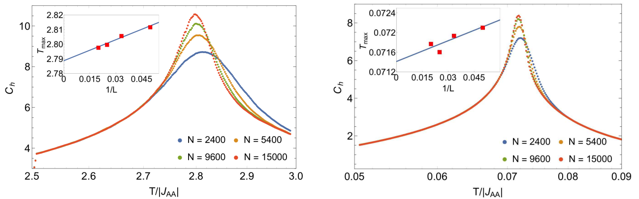
FIG. 9. Finite size effects on the specific heat for x = -3 (left) and x = -1.05 (right). Insets: The transition temperature is scaled as a function of 1/L where L is the linear system size. In the thermodynamic limit, we find T_c = 2.788(5) for x = -3 and T_c = 0.0714(5) for x = -1.05
