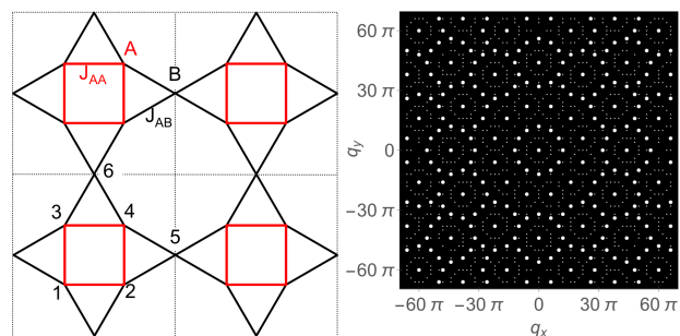
FIG. 1. The shuriken lattice as seen in real space ( left ) and Fourier space ( right ). There are 6 sites per unit-cell with two sublattices A and B . Interactions between A-sites (square plaquettes) are described with coupling constant J_{AA} (red), while interactions between A- and B-sites (octagonal plaquettes) are described with J_{AB} (black).
