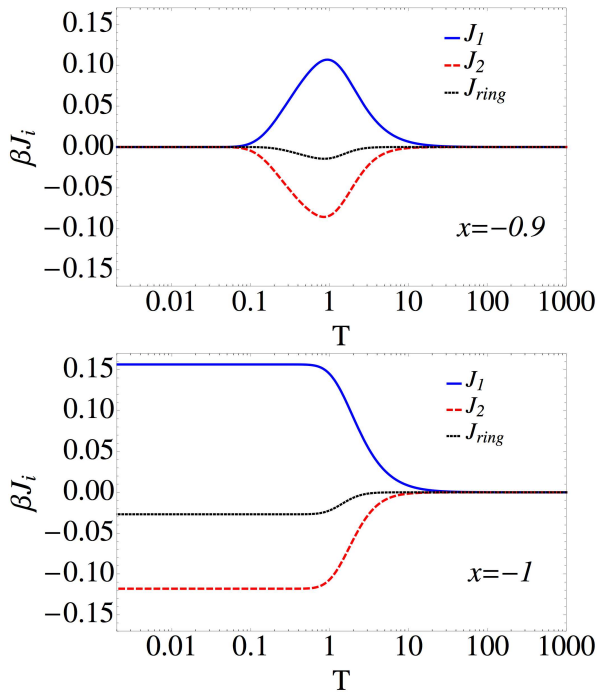
FIG. 5. Behavior of the coupling constants of the the effective checkerboard lattice model as a function of temperature [Eq. (12)] for x = -0.9 (upper panel) and x = -1 (lower panel). Upper panel: All couplings vanish at both high and low temperatures with an intermediate regime at T \sim 1 where the effective interactions are stronger. The intermediate regime corresponds to the spin liquid region of the phase diagram Fig. 2, with the high- and low-temperature regimes corresponding to the paramagnet and binary paramagnet respectively. Lower panel: For all couplings \mathcal{J}_i , \beta\mathcal{J}_i vanishes at high temperature and tends to a finite constant of magnitude |\beta\mathcal{J}_i(T)| \ll 1 at low temperature. The short range correlated, spin-liquid regime, thus extends all the way down to T = 0 .
