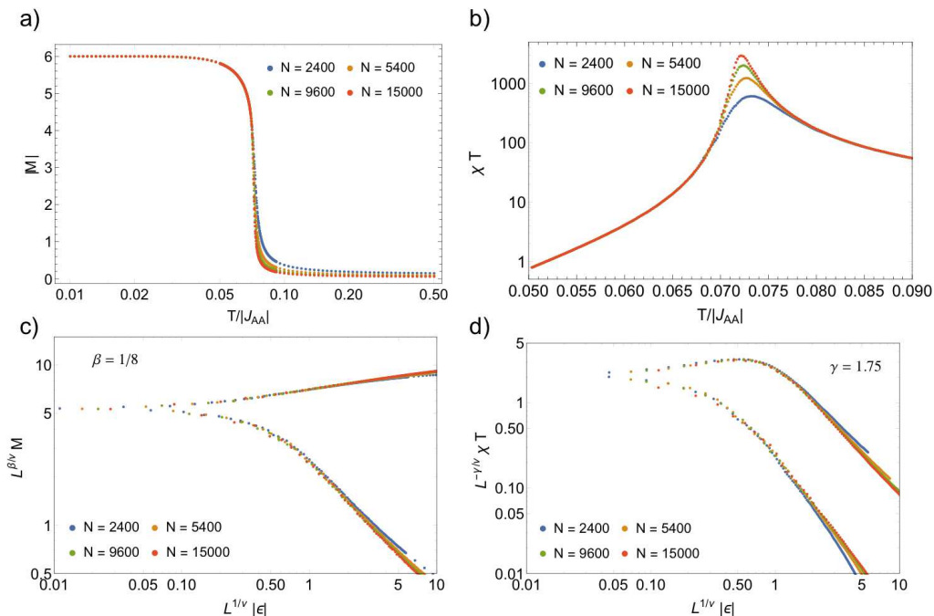
FIG. 11. Finite size scaling of the magnetization |M| (a,c) and susceptibility \chi (b,d) for x = -1.05 .
