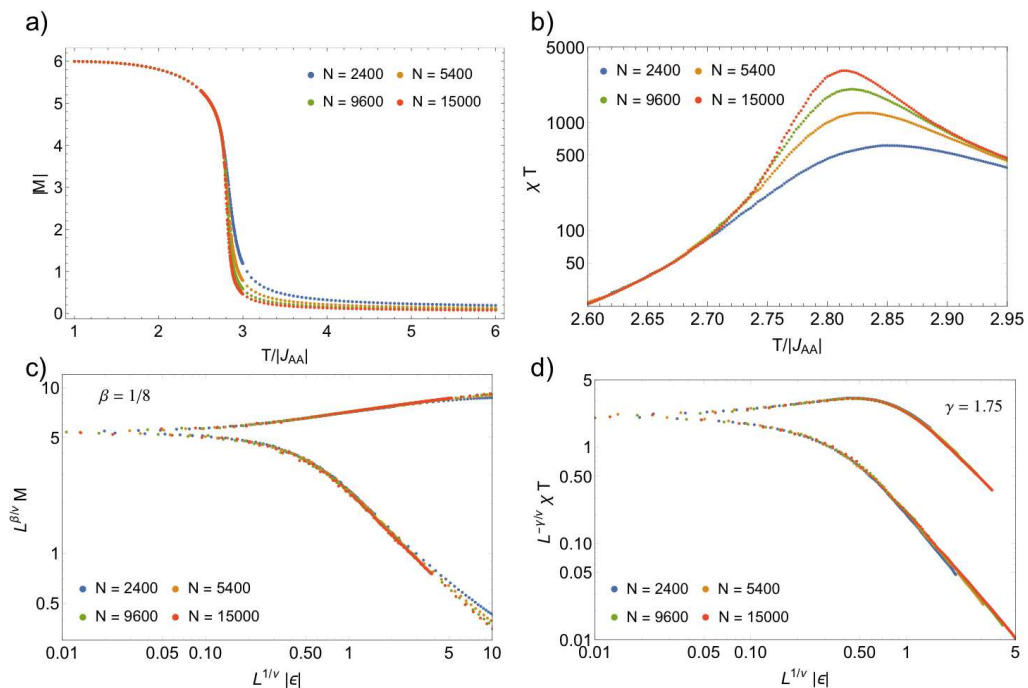
FIG. 10. Finite size scaling of the magnetization |M| (a,c) and susceptibility \chi (b,d) for x = -3 .
