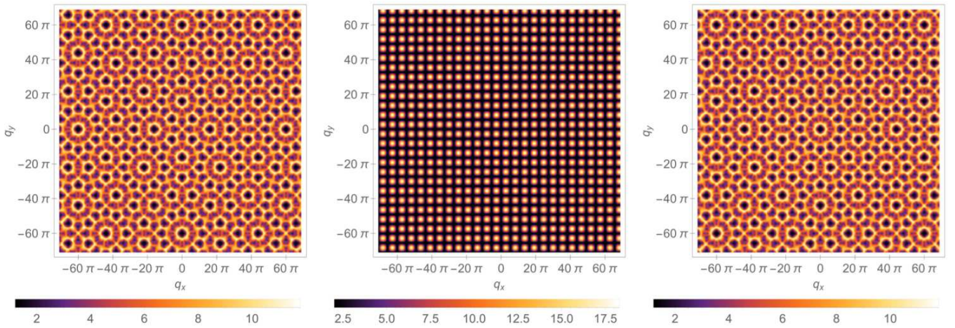
FIG. 8. Static structure factors of the anisotropic shuriken lattice for (a) x = -1 , (b) x = 0 and (c) x = 1 at zero temperature, obtained from Monte Carlo simulations. For x = \pm 1 , the scatterings are strongly inhomogeneous (as opposed to a standard paramagnet) and non-divergent ( i.e. without long-range order), confirming the spin liquid nature of these phases. The structure factors of the x = +1 and x = -1 models are similar by a (q_x, q_y) = (60\pi, 0) or (0, 60\pi) translation. The patterns are related to the 6-site unit cell of the shuriken lattice, as visible from Fig. 1. On the other hand for (b) x = 0 , the black background underlines the absence of correlations in the binary paramagnet beyond the size of the superspins (square plaquettes), which is responsible for the finite extension of the dots of scattering. In order to restore ergodicity, a local update flipping the four spins of square plaquettes was used in the simulations. A video showing the temperature dependence of the static structure factor for x = 0.9 is available in the Supplementary Materials.
