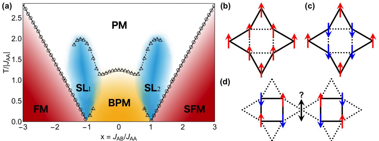
FIG. 2. Phase Diagram of the Ising model on the anisotropic shuriken lattice. (a) The circles (triangles) correspond to phase transitions (crossovers), obtained by Monte Carlo simulations (Husimi-tree calculations) [see appendix A for further details]. As a function of the coupling ratio x = \frac{J_{AB}}{J_{AA}} , the model supports a long-range ordered ferromagnet (FM) [see panel (b)], a long-range ordered staggered ferromagnet (SFM) [see panel (c)], a binary paramagnet (BPM) [see panel (d)], and two classical spin liquids (SL 1,2 ). The BPM illustrated in panel (d) is made of antiferromagnetically ordered square plaquettes, decoupled from each other and from the intermediate spins sitting on the B sublattice. For |x| \gtrsim 1 , on cooling, the system undergoes an evolution from “gas \xrightarrow{\text{crossover}} liquid \xrightarrow{\text{transition}} solid”. As for |x| \lesssim 1 , it provides a remarkable example of reentrance from “gas \xrightarrow{\text{crossover}} liquid \xrightarrow{\text{crossover}} gas”.
