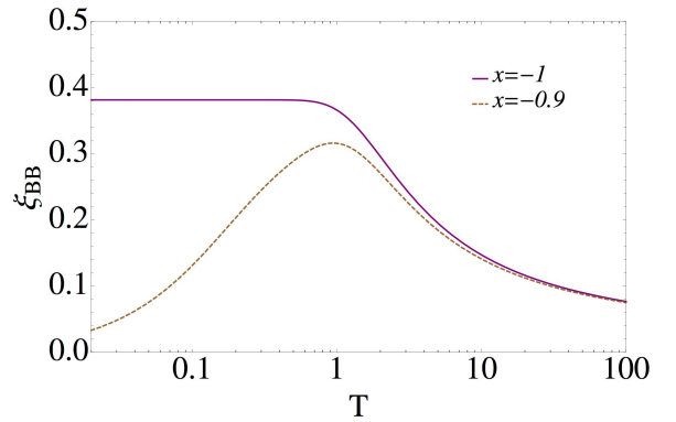
FIG. 6. Correlation lengths in the effective checkerboard model , calculated from Eq. (15), for x = -0.9 and x = -1 . The correlation length is calculated to leading order in a perturbative expansion of the effective model in powers of \beta\mathcal{J}_i . Such an expansion is reasonable for |x| \leq 1 since \beta\mathcal{J}_i \ll 1 for all T (see Fig. 5). For x = -0.9 the behavior of the correlation length is non-monotonic. The correlation length is maximal in the spin liquid regime but correlations remain short ranged at all temperatures. In the binary paramagnet regime, the correlation length vanishes linearly at low temperature. For x = -1 , the correlation length enters a plateau at T \sim 1 , and short range correlations remain down to T = 0 .
