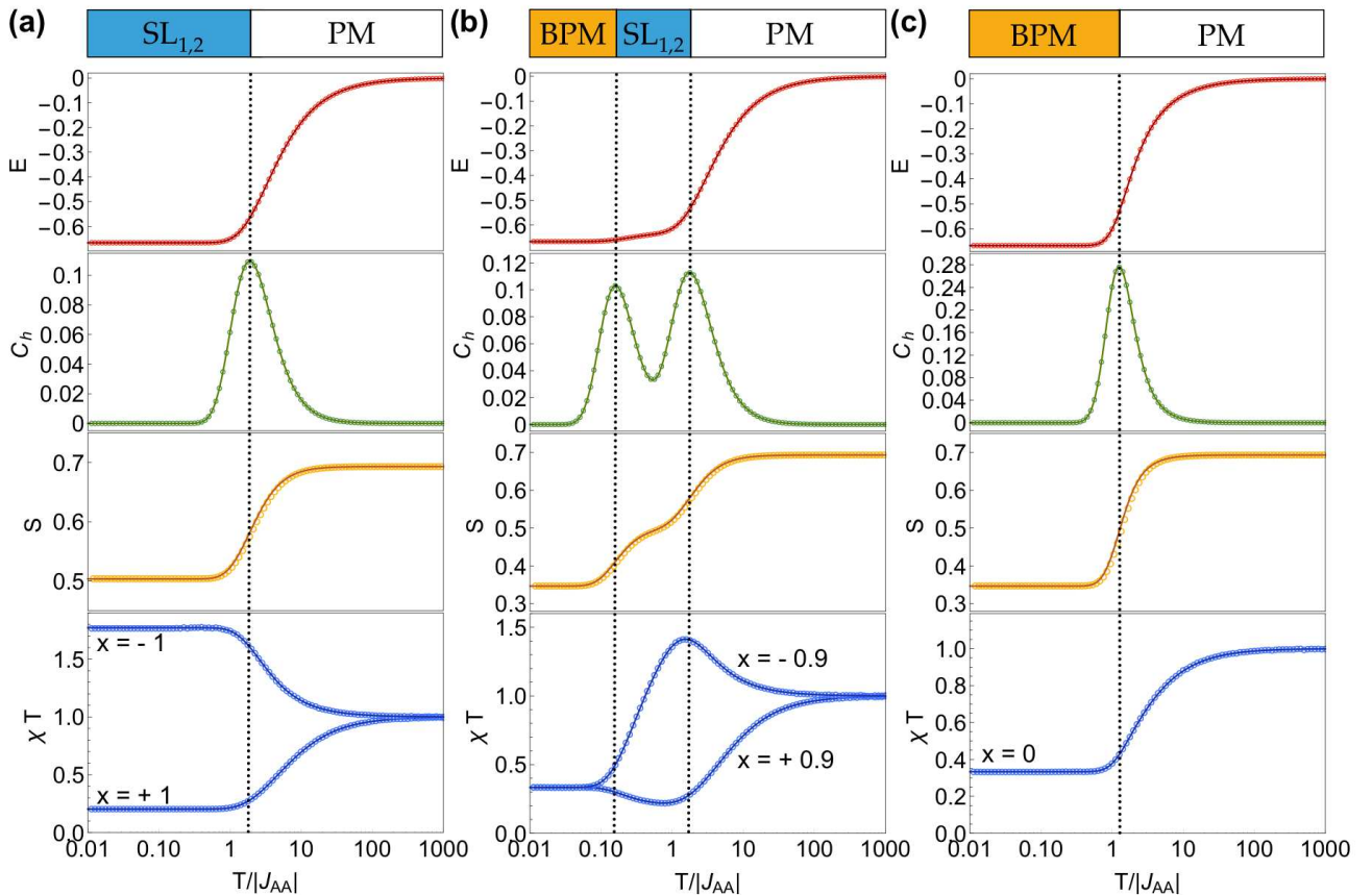
FIG. 3. Multiple crossovers between the paramagnetic, spin-liquids and binary regimes as observed in the specific heat C_h , entropy S and reduced magnetic susceptibility \chi T . The models correspond to a) x = \pm 1 , b) x = \pm 0.9 and c) x = 0 . There is no phase transition for this set of parameters, which is why the Husimi tree calculations (lines) perfectly match the Monte Carlo simulations (circles) for all temperatures. The double crossover is present for x = \pm 0.9 , with the low-temperature regime being the same as for x = 0 , as confirmed by its entropy and susceptibility. The entropy is obtained by integration of C_h/T , setting S(T \rightarrow +\infty) = \ln 2 . The vertical dashed lines represent estimates of the crossover temperatures determined by the local specific-heat maxima. The temperature axis is on a logarithmic scale. All quantities are given per number of spins and the Boltzmann constant k_B is set to 1.
