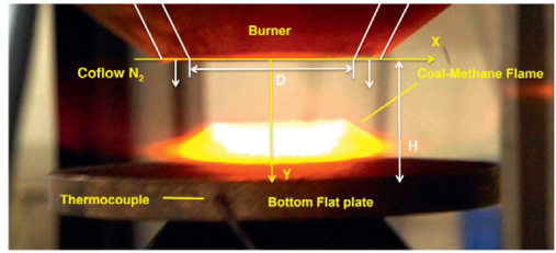
Fig. 1. Direct view of coal/methane/air flame.
