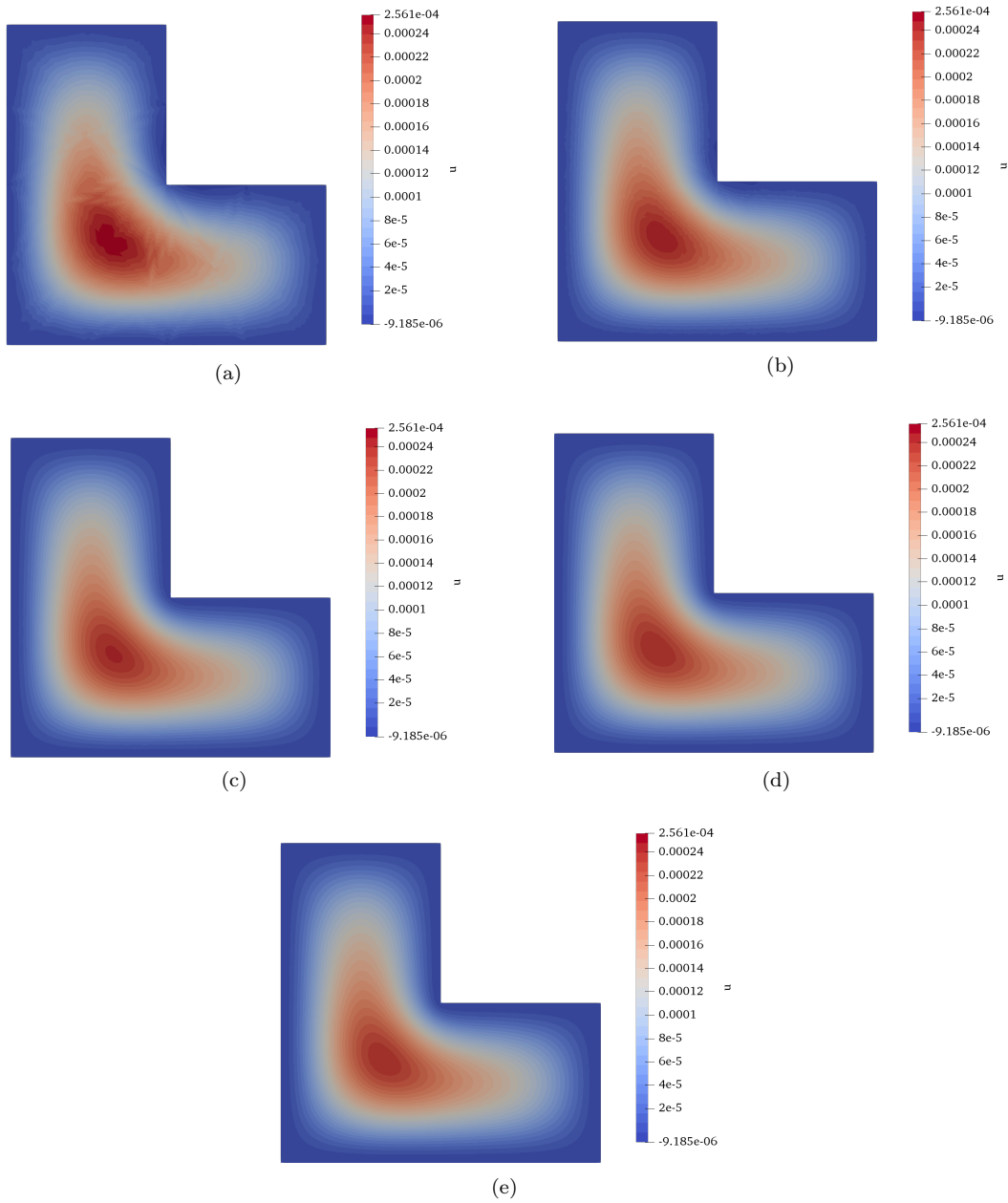
Figure 6: Numerical solution obtained for a uniform load f \equiv 1 , on five uniformly refined triangular meshes (with N elements) of the domain, with k = 3 . Case (a): N = 34 ; case (b): N = 136 ; case (c): N = 544 ; case (d): N = 2176 ; case (e): N = 8704 .
