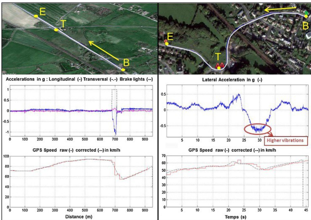
Fig. 3 Longitudinal Incident with emergency braking (Left) and lateral Incident in a tight curve (Right): trajectory on the site, accelerations, speed .
