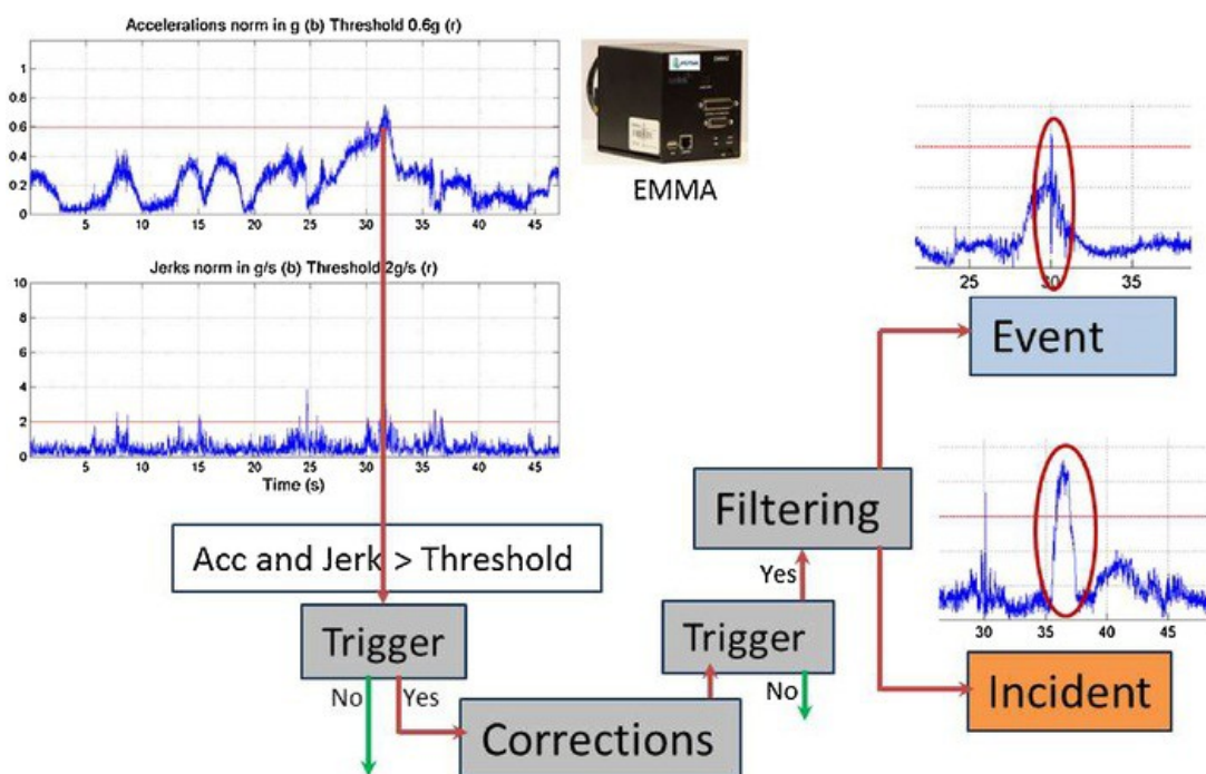
Fig. 1 Principle of classification for simple events and genuine incidents.
