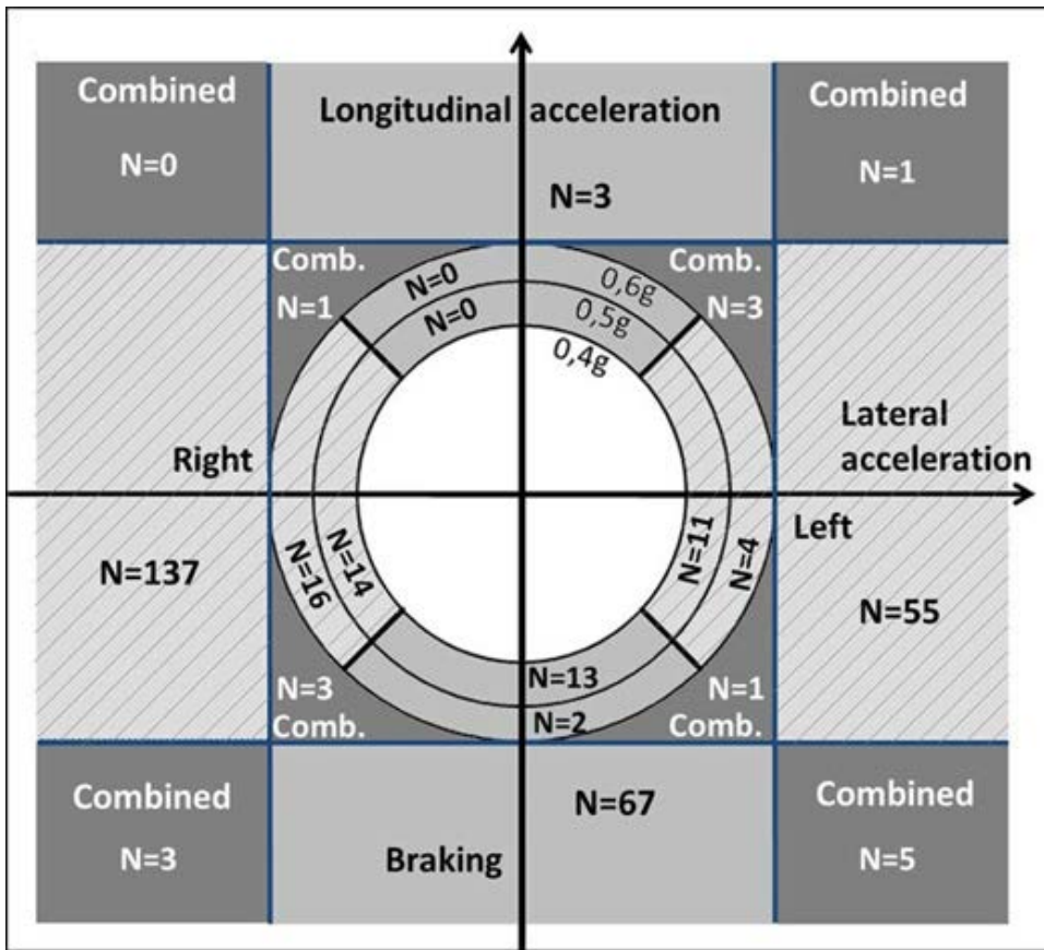
Fig. 4 Distribution of incidents according to the main dynamical demands on the vehicle.
