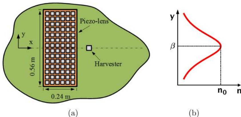
Fig. 1. (a) The harvesting system with piezo-lens and (b) the gradient variation profile of the refractive index n(y) .
