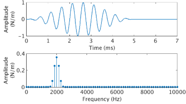
Figure 4: The applied tone burst excitation.
