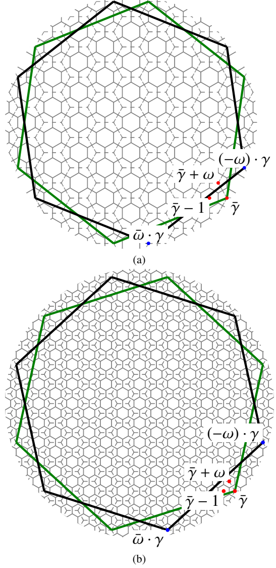
Fig. 8 Visualization of C_{\gamma \cdot (2+\omega)}(0) and C_{\bar{\gamma} \cdot (2+\omega)}(0) for: s = 3, t = 5 (a); s = 4, t = 9 (b), depicted in black and green, respectively. The usual hexagonal grid is depicted in gray, whereas its mapping by 2 + \omega is depicted in gray and represented by dashed line segments
