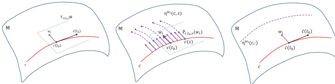
Figure 1: Exp-parallelization on a schematic manifold. Left: a non-zero vector \mathbf{w}_i is chosen in T_{c(t_0)}\mathbb{M} . Middle: the tangent vector \mathbf{w}_i is transported continuously along the curve c . Then, a point \eta^{\mathbf{w}_i}(c, s) is constructed at time s by use of the Riemannian exponential. Right: The curve \eta^{\mathbf{w}_i}(c, \cdot) is the “parallel” resulting from the construction.
