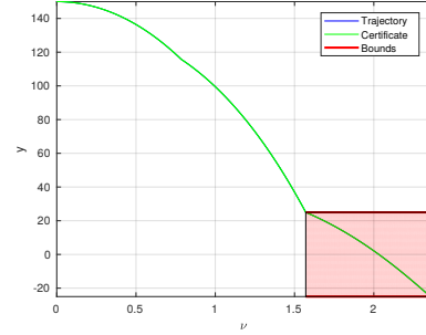
(b) Y-trajectory, RPAs of degree 7.
