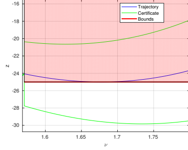
(c) Excursion of z-trajectory, RPAs of degree 5.
