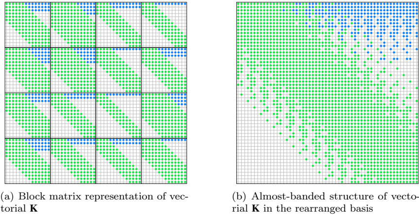
Fig. 2 Two representations of vectorial integral operator \mathbf{K}
