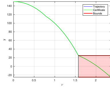
(a) Y-trajectory, RPAs of degree 5.
