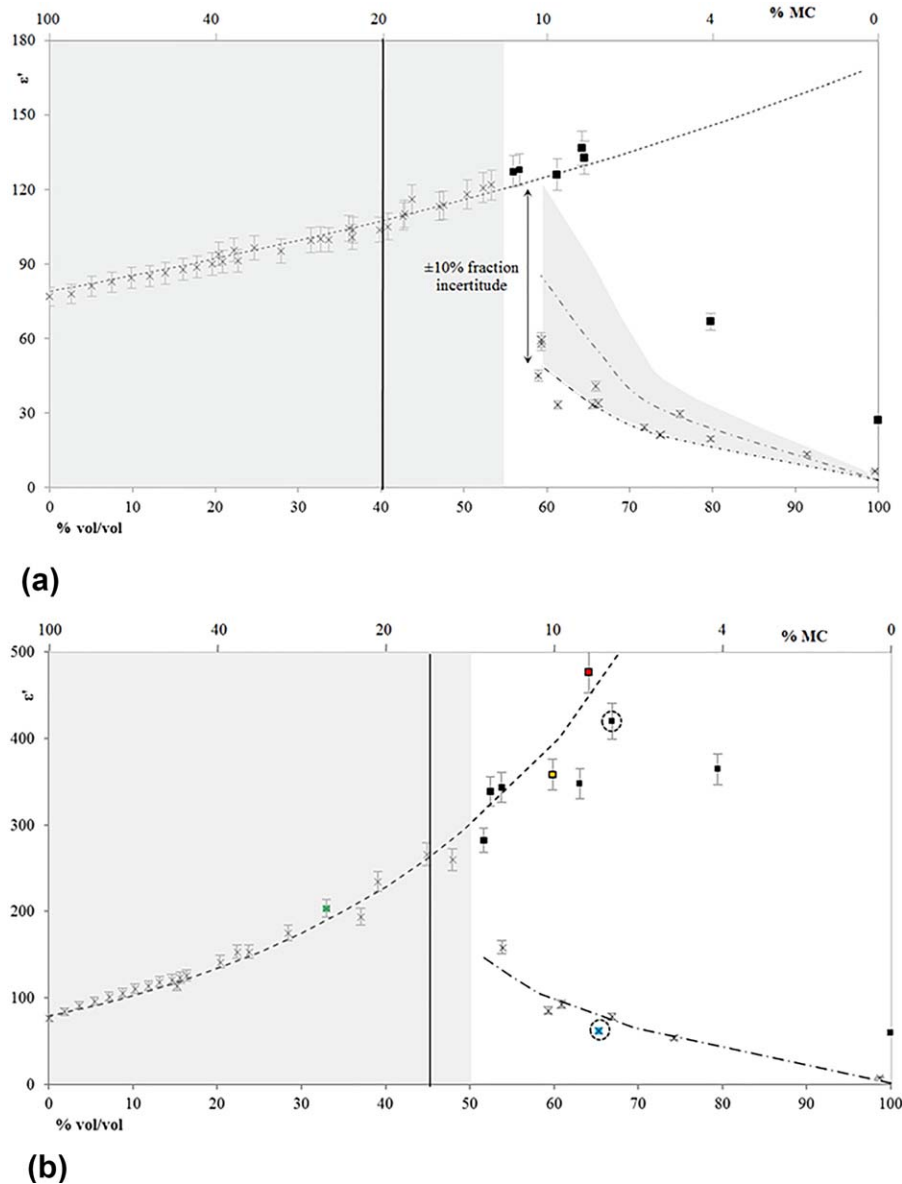
FIG. 4. Real part of permittivity as a function of water content (% v/v on the bottom horizontal axis and % MC on the top horizontal axis) at 300 MHz, for \text{CaTiO}_3 (a) and \text{BaTiO}_3 (b) solutions manually (x) and machine-pressed (■), as well as the two-phase Lichtenecker's logarithmic power law (----) represented at the first stage (gray area), and three-phase CPA law (- · -) represented at the second stage (white area). The black vertical lines refer to the maximal water content reported in the literature (21). In the case of \text{CaTiO}_3 , the CPA law is shown calculated with the original air and powder fractions (dashed gray curve), and also calculated by taking into account a \pm 10\% uncertainty associated with the measurement devices, which influence the air and powder fractions. When considering a 10% reduction in the air fractions (dashed and dotted black curve), the CPA law is found to agreeably integrate the experimental data. The two dashed circles represent the samples shown in Figure 2d. The four colored points correspond to the pads tested in the 7T MRI (corresponding to the colored frames in Fig. 6c).
