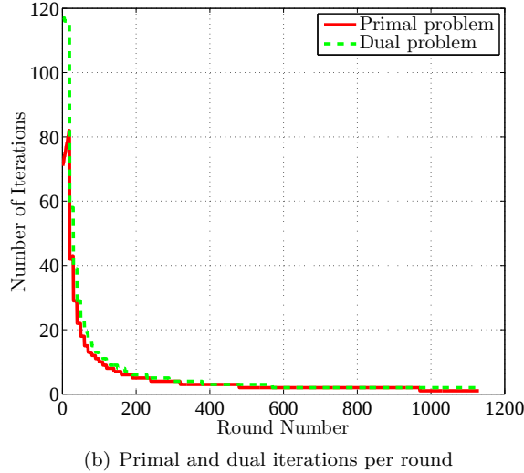
Figure 1: Primal variables and number of iterations
