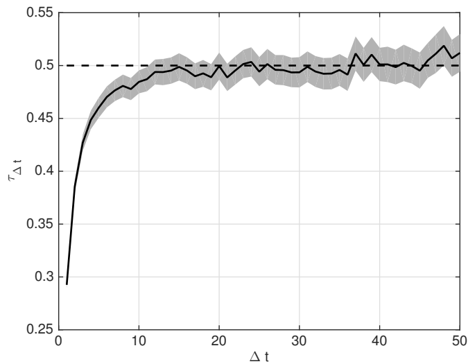
FIG. 5. Plot of the estimated correlation time \tau_{\Delta t} (black line) and error bars (grey shading) as functions of \Delta t . For small values of \Delta t , the large-time limit in (35) is not achieved, which explains the low values of \tau_{\Delta t} . For too large values of \Delta t , the empirical average \mathbb{E}_{\frac{T}{\Delta t}} in (38) is not accurate due to the small value of \frac{T}{\Delta t} , which explains the increasing fluctuations in \tau_{\Delta t} as \Delta t increases. The optimal value \Delta t^* is the one in between these artificial behaviour. Here, one can read \Delta t^* \simeq 20 and \tau_{\Delta t^*} \simeq 0.5 , in agreement with the exact value \tau = 1/2 (dashed line). The Ornstein-Uhlenbeck process (36) has been integrated over T = 5.10^4 using the method proposed in Ref. 38, with time step 10^{-3} .
