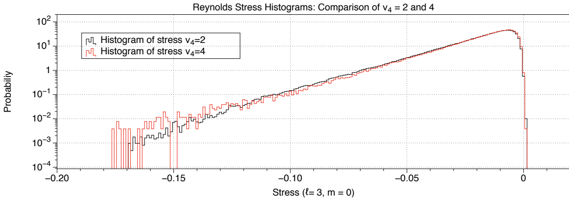
FIG. 3. Probability density functions of R_3 , the third component in the spherical harmonics decomposition of the zonally averaged advection term R(\phi) , from direct numerical simulations of the quasi-linear barotropic equation (12) with hyper-viscosity such that the smallest scale has a hyperviscous damping rate of 4 (red curve) and 2 (black curve). Both probability density functions are similar, showing that hyper-viscosity can be considered to be negligible in zonal jet statistics.
