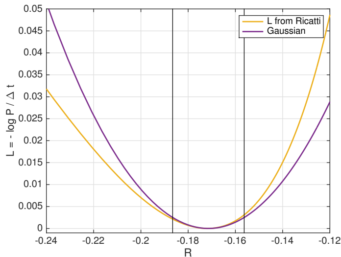
FIG. 12. Yellow curve: large deviation rate function \mathcal{L}_{10,3}(\bar{R}) computed from numerical integration of the Ricatti equation (34), using (33) and (48), with parameters defined in section II B and \alpha = 0.073 . Purple curve: quadratic fit (55) that corresponds to a Gaussian process with same mean and variance as \bar{R}_{10,3,\Delta t} , the time-averaged advection term. Black vertical lines: standard deviation of \bar{R}_{10,3,\Delta t} around its mean. Outside those vertical lines, we observe non-Gaussian behaviour of \bar{R}_{10,3,\Delta t} , in particular negative fluctuations are much more probable than positive ones.
