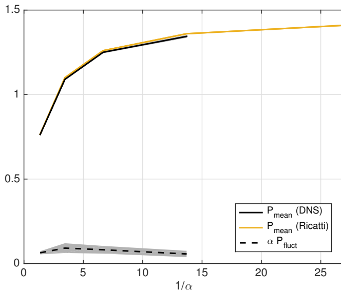
FIG. 7. Total energy injection rate into the zonal flow by the mean Reynolds' stresses P_{mean} (first term in the r.h.s of (43), in solid line) and by the fluctuations of Reynolds' stresses \alpha P_{fluct} (last term in the r.h.s of (43), in dashed line with statistical error bars in grey shading) as a function of 1/\alpha . Those quantities are estimated from direct numerical simulations (DNS) of the linearized barotropic equation (49) with parameters given in section II B, and P_{mean} is also computed directly using the Ricatti equation (34) (yellow curve).
