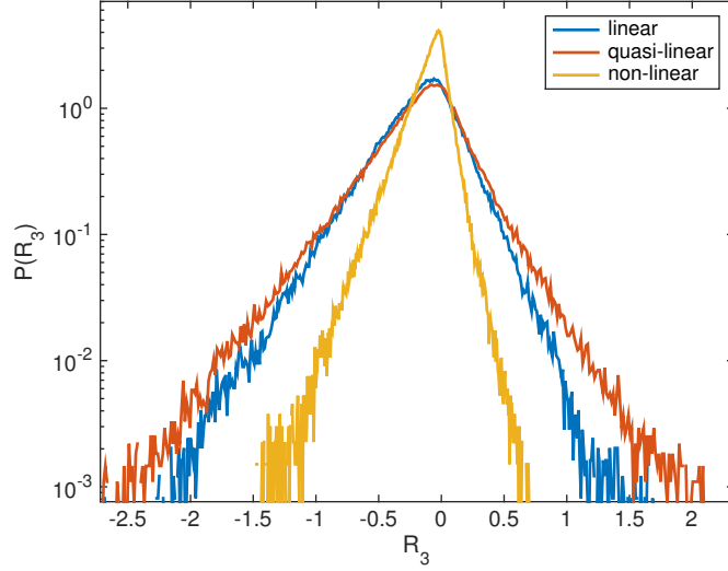
FIG. 2. Probability density functions of R_3 , the third component in the spherical harmonics decomposition of the zonally averaged advection term R(\phi) , from direct numerical simulations of the linear barotropic equation (14) (blue), the quasi-linear barotropic equation (12) (orange), and the non-linear barotropic equation (10) (yellow). Exponential tails are observed in all of those different cases. The common parameters are \alpha = 0.073 , \Omega = 3.7 , total integration time 5,450, and the forcing is concentrated in wavenumbers |m| = 10 , \ell = 10 .
