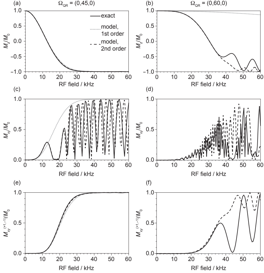
FIG. 3: Simulations of the RF inversion and refocussing profiles of an S^3 AP applied to two single-crystal orientations of a spin I = 1 subject to a quadrupolar interaction. The crystallite orientation (0^\circ, 45^\circ, 0^\circ) has sideband parameters B_q^{(0)} = 0.16 and c_\Sigma = -0.21 , and the orientation (0^\circ, 60^\circ, 0^\circ) has B_q^{(0)} = 0.01 and c_\Sigma = -0.37 . The two RF inversion profiles, shown in (a) and (b), plot the expectation value of \hat{I}_z , M_z/M_0 , as a function of RF field amplitude following a single WURST-20 pulse applied to the centreband. In plot (a) complete inversion is obtained with RF field amplitudes above 40 kHz, where the adiabaticity factors in regimes A and B are Q_A^{(1)} = 4.37 and Q_B^{(1)} = 0.39 , indicating that the pulse is operating in regime A. By contrast in plot (b) complete inversion is obtained with RF field amplitudes above 60 kHz, where Q_A^{(1)} = 0.04 and Q_B^{(1)} = 6.44 , indicating that the pulse is operating in regime B. The corresponding single-quantum RF refocussing profiles, shown in (c) and (d) plot the expectation value of \hat{I}_- , M_{xy}/M_0 , following the application of a pair of the same WURST-20 pulses to the centreband. In this case the coherence-transfer pathway has been filtered to select p = -1 \rightarrow +1 \rightarrow -1 . The plots in (e) and (f) are double-quantum RF refocussing profiles, which show the expectation value of \hat{I}_-^{(+1,-1)} , M_{xy}^{(+1,-1)}/M_0 , following the application of the pair WURST-20 pulses. Here the selected coherence-transfer pathway is p = -2 \rightarrow +2 \rightarrow -2 . The results for the crystallite orientation specified by \Omega_{QR} = (0^\circ, 45^\circ, 0^\circ) are shown in (a), (c), and (e), and those for \Omega_{QR} = (0^\circ, 60^\circ, 0^\circ) are shown in (b), (d), and (f). The solid black curves correspond to the exact simulations. The results computed from the jolting-frame approximation are also shown. The dotted grey curves show the results calculated using the first-order effective Hamiltonian (equations 91 and 92), and the dashed black curves show the results calculated from the effective Hamiltonian up to second order (equations 91, 92, 94, and 95). The quadrupole parameters are C_Q = 1.19 MHz ( \omega_Q/2\pi = 892.5 kHz) and \eta_Q = 0.52 , and the MAS frequency is 60 kHz. The WURST-20 pulse [11] is of 1 ms duration and sweep width 60 kHz, and is applied to the centreband.
