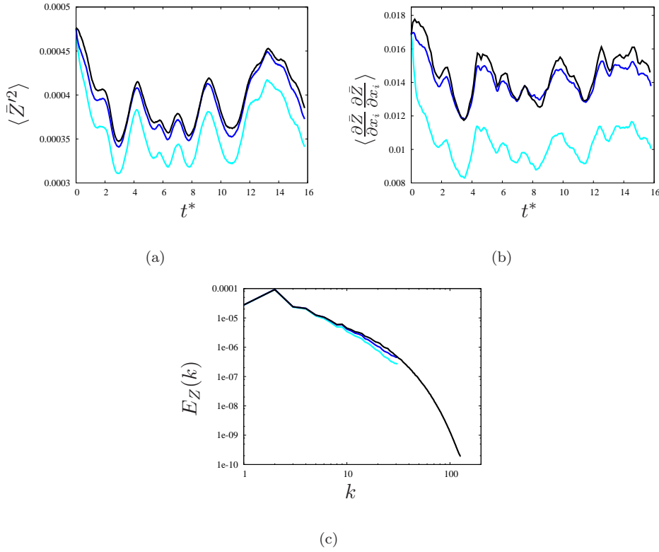
Figure 10. Forced scalar case: evolution of the resolved scalar variance (a) and scalar enstrophy (b) with time, and scalar variance spectrum (c). The models are compared with filtered DNS (a,b) or full DNS (c). DNS (black line), DED model (cyan line) and AC model (blue line).
