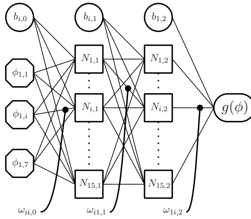
Figure A1. ANN topology used for training.
