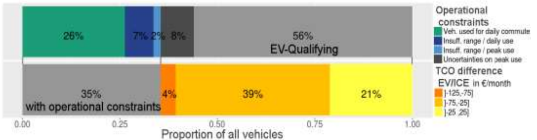
Figure 5: Projected constraints analysis for eLCVs compared to conventional LCVs, in 2021
