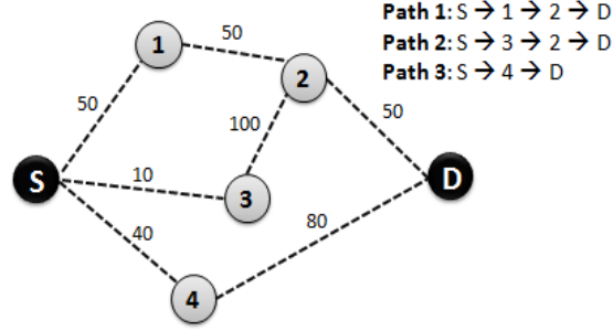
Fig. 1. An illustrative example to demonstrate the effectiveness of Opt-FLQE RM metric.
