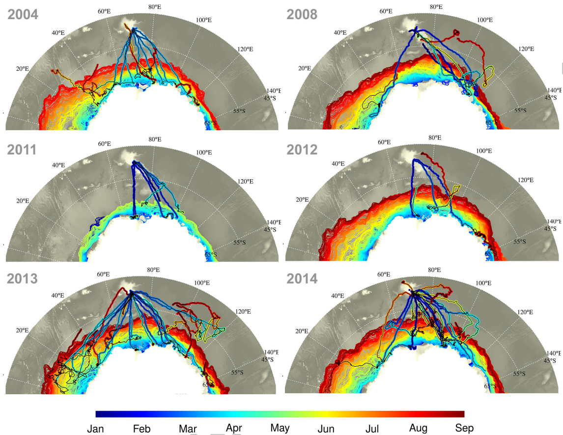
Fig 3. Tracks of the 46 post-moulting individuals equipped with CTD-SRDs from 2004 to 2014, linked with the seasonality of the sea ice in the East Antarctic region. The colour scale represents the time and the same colour is used for sea ice extent and tracks of animals; the sea ice extent of a given day and associated seal positions are colored in the same way. For visual purposes, tracks and sea ice extent were limited to September (annual maximum sea ice extent) and the unique individual in 2009 was removed. For all years, sea ice extent was obtained from SSM/IS daily sea ice concentration (resolution 25 km).
