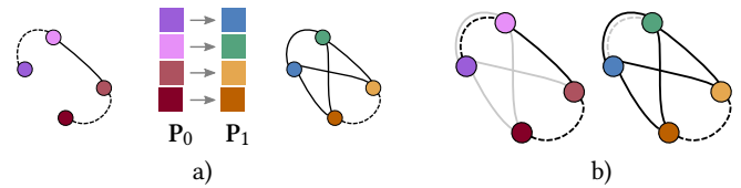
Fig. 5. Hypergraph symmetrization. a) Two input constrained palettes with different hypergraphs, composed by contrast and component-wise differences constraints, represented respectively as plain and dashed lines. b) Adapted constraint graphs, dummy edges are shown in gray.
