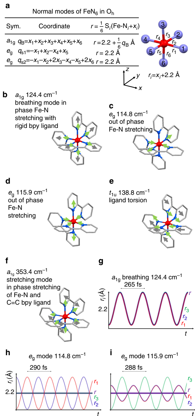
Figure 3 | HS normal modes. (a) Fe-N bond coordinate and average length r for a_{1g} and e_g symmetry normal modes. (b-f) Respective representation of normal breathing mode (124.4 cm -1 , in-phase stretching of the 6 Fe-N i bonds with almost rigid bpy ligands), the global stretching mode (353.4 cm -1 , bpy and Fe-N stretching), stretching modes at 114.8 and 115.9 cm -1 and a bending mode at 138.8 cm -1 . Green arrows show N motions and grey ones ligand motions. (g-i) Time evolution of the symmetry independent bonds r_1 , r_2 and r_3 with respect to inversion symmetry and their average r (purple).
