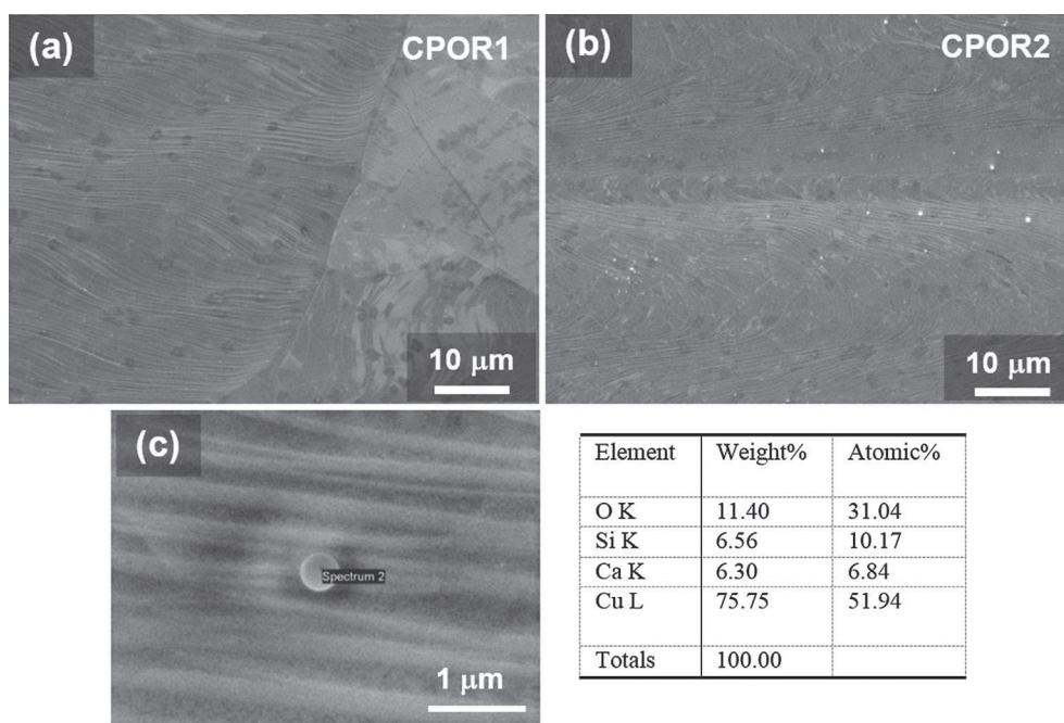
Fig. 6. FEG-SEM micrographs of graphene films grown on 'CPOR' foil using (a) 300 sccm H 2 flow (CPOR1 sample) and (b) 200 sccm Ar/100 sccm H 2 (CPOR2 sample) during heating. (c) EDX analysis result of a spherical impurity nanoparticle observed in (b).
