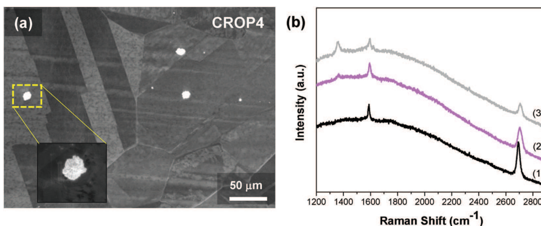
Fig. 2. (a) FEG-SEM micrograph of the graphene film grown on 'CROP' foil using 200 sccm Ar flow during heating (CROP4 sample). Inset shows higher magnification of the impurity particle indicated by a dashed rectangle. (b) Raman spectra recorded at different spots on the CROP4 sample showing (1) Monolayer graphene, (2) Bilayer graphene and (3) Few-layer (3–5 layers) graphene. (A color version of this figure can be viewed online.)
