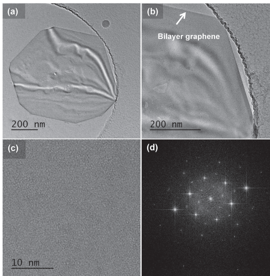
Fig. 9. (a), (b) Low magnification TEM and (c) HRTEM images of a bilayer graphene island on the CPOR3-NA sample and (d) FFT of the corresponding HRTEM image shown in (c).
