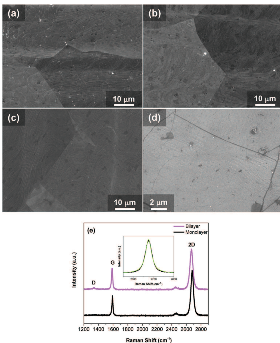
Fig. 8. FEG-SEM micrographs of graphene films grown on 'CPOR' foil using (a) 200 sccm Ar/100 sccm H 2 during heating and 100 sccm H 2 /17 sccm CH 4 gas flow during graphene growth (CPOR3 sample), (b) the same process conditions as indicated in (a), but at a 0.3 and 0.2 Torr during heating and annealing, instead of 0.5 Torr. The Cu foil was mechanically cleaned prior to acetic acid cleaning (CPOR3-MC sample), and (c) the same conditions as indicated in (b), but the Cu foil was pre-cleaned in a nitric acid solution for 60 s instead of acetic acid (CPOR3-NA sample). (d) FEG-SEM micrograph of the CPOR3-NA sample transferred onto a SiO 2 (300 nm)/Si substrate. (e) Representative Raman spectra recorded at different spots across the CPOR3-NA sample. Inset shows the single Lorentzian fit of the 2D-band of monolayer graphene. (A color version of this figure can be viewed online.)
