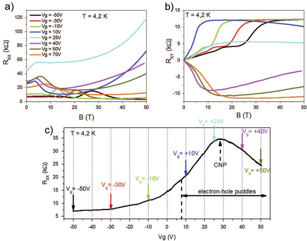
Fig. 10. (a) Longitudinal ( R_{XX} ) and (b) Hall ( R_{XY} ) resistance of the CPOR3-NA sample measured as a function of magnetic field of up to 50 T, for various values of the back-gate voltage. (c) Zero-field resistance of the CPOR3-NA sample measured at 4.2 K as a function of the back-gate voltage. The arrows indicate the back-gate voltages at which high magnetic field measurements have been performed (e.g., (a) and (b)). The horizontal arrow indicates the back-gate voltage range in which both electron and hole coexist. (A color version of this figure can be viewed online.)
