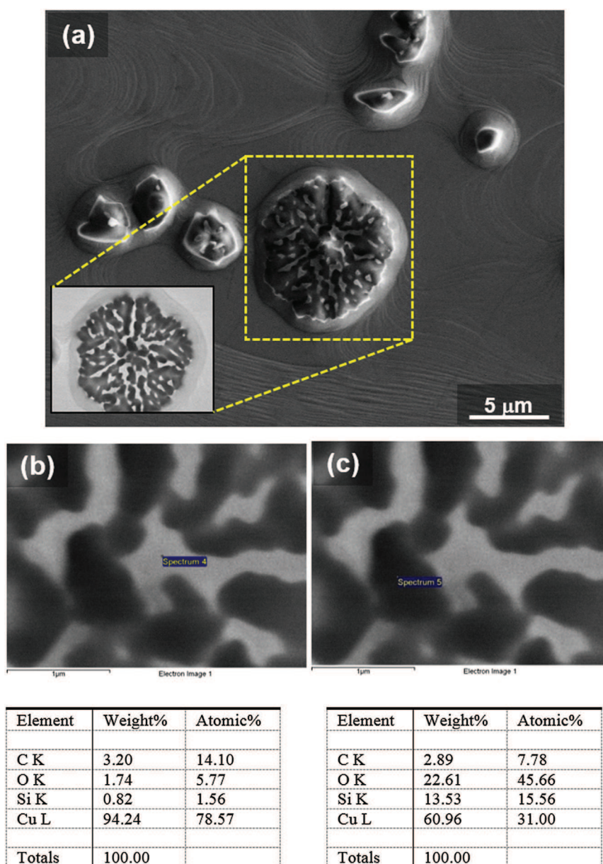
Fig. 3. (a) Secondary electron image of impurities observed on the CROP4 sample. Inset shows the BSE image of the impurity particle indicated by a dashed rectangle, revealing the presence of two different phases. (b), (c) EDX analysis results of these two phases. (A color version of this figure can be viewed online.)
