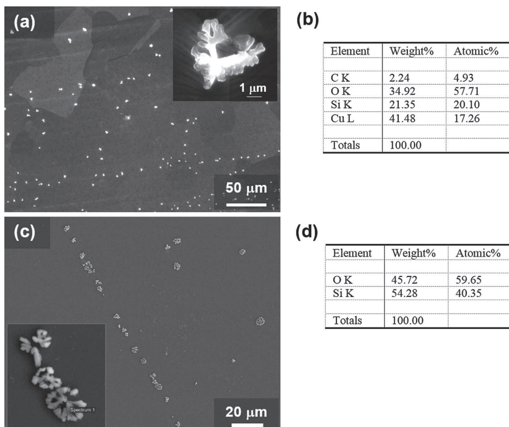
Fig. 5. (a) FEG-SEM micrograph of the CPOR4 sample on Cu foil, revealing the impurity particles on the surface. Inset shows higher magnification of an impurity particle. (b) EDX result of the corresponding impurity particle shown at the inset in (a). (c) FEG-SEM micrograph of CPOR4 sample transferred onto a SiO 2 (300 nm)/Si substrate. The impurity particles were also transferred together with the graphene film. (d) EDX analysis result of an impurity particle (shown at the inset in (c)).
