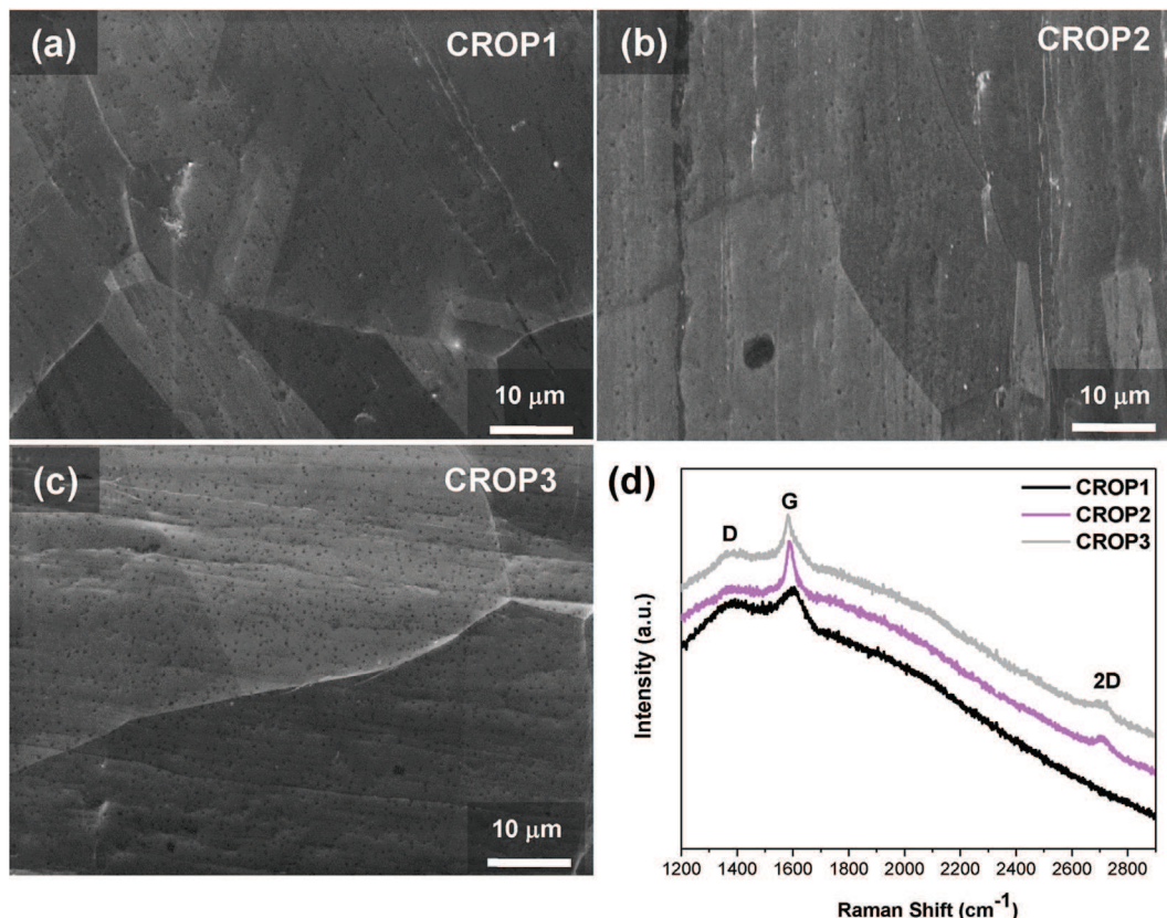
Fig. 1. FEG-SEM micrographs of ‘CROP’ foil after being subjected to CVD growth process under different heating conditions (a) 300 sccm H 2 heating (CROP1), (b) 200 sccm Ar/100 sccm H 2 heating (CROP2), and (c) Hot loading the foil into a preheated furnace at 1000 °C for annealing step (CROP3). (d) Raman spectra of the samples shown in (a), (b) and (c). (A color version of this figure can be viewed online.)
