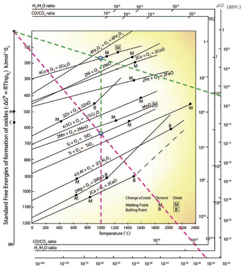
Fig. 7. Standard free energies of formation of oxides as a function of temperature 1 [23]. (A color version of this figure can be viewed online.)
