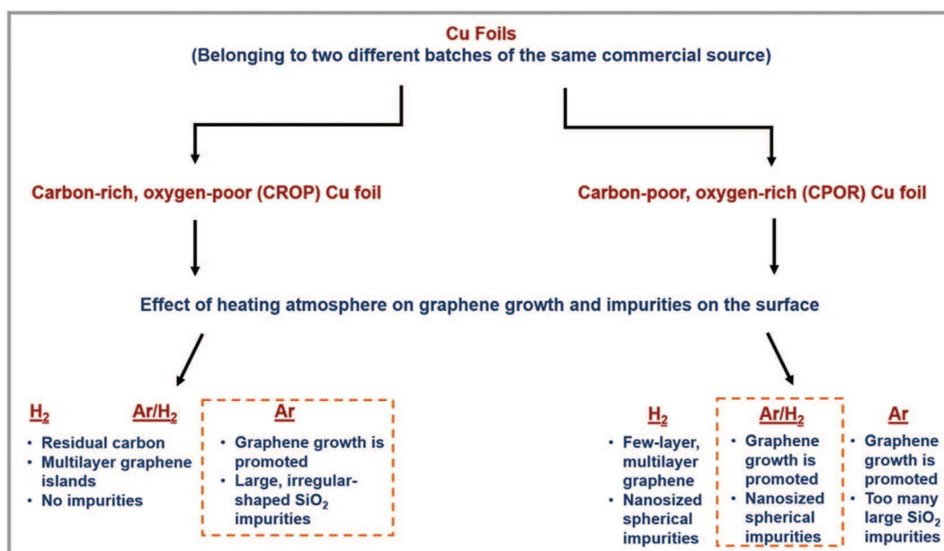
Fig. 11. Summary of the relationship between heating atmosphere and Cu foil impurities during graphene growth via low pressure CVD. (A color version of this figure can be viewed online.)
