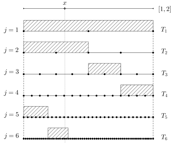
FIG. 1 : Construction of the first terms of (\zeta_k)_{k \geq 0} . The hatched zone corresponds to the values of x for which \zeta_{[2^j x]} takes nonzero values.
