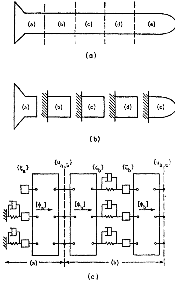
FIG. 4. Dynamic partitioning of missile structure. (a) Missile structure, unpartitioned. (b) Support conditions for partitions while calculating substructure vibration modes. (c) Portion of composite model.
