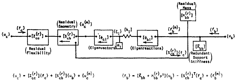
FIG. 5. Improved representation of a substructure for the general case.
