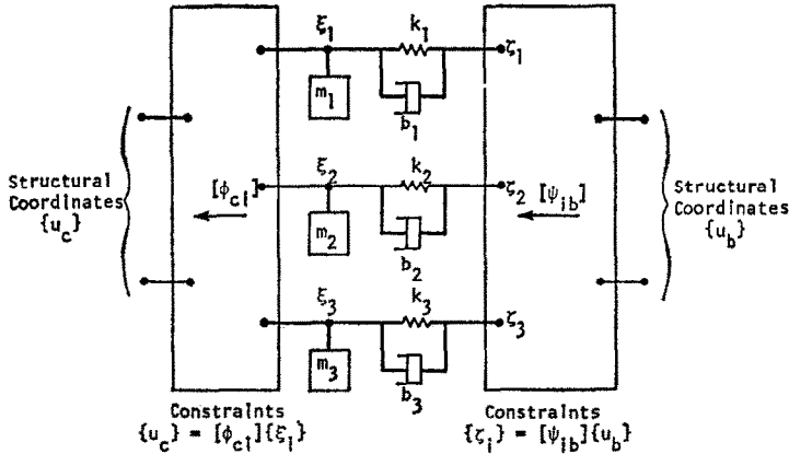
FIG. 3. Representation of part of a structure by its vibration modes in the general case when some connection points are free and some are rigidly constrained.
