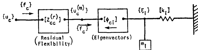
FIG. 6. Improved representation for case in which all connection coordinates are free in modal calculation.
