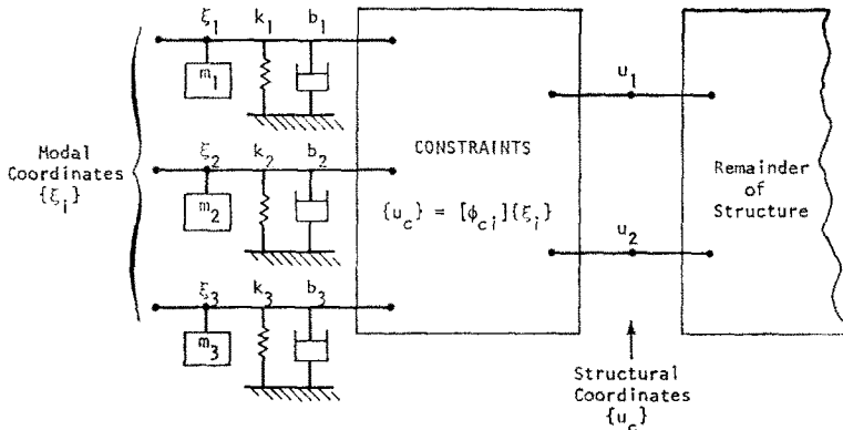
FIG. 2. Representation of part of a structure by its vibration modes when all connection points are free while the modes are calculated.
