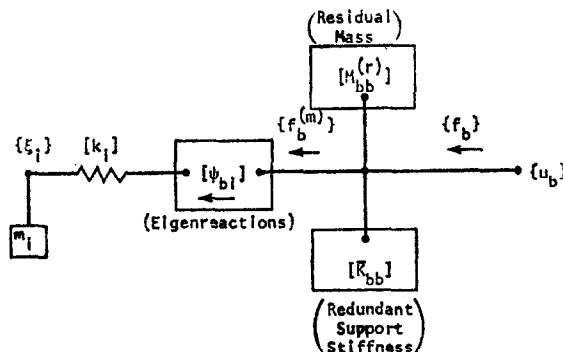
FIG. 7. Improved representation for case in which all connection coordinates are constrained in modal calculation.
