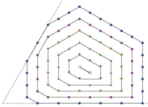
Figure 1: The Horn-tensor polygon \tilde{\mathbf{H}}_{\alpha\beta} = \mathbf{H}_{\lambda\mu} for the two SU(3) weights \lambda = (9, 5) \mu = (6, 5) , hence \alpha = (14, 5, 0) , \beta = (11, 5, 0) . The multiplicity increases from 1 to 6 inside the polygon, giving a matriochka pattern to the successive contours.
